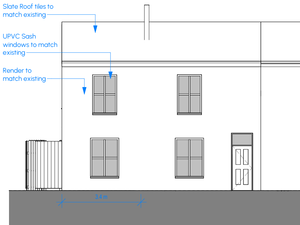
Planning - Proposed Front Elevation A 1:100
