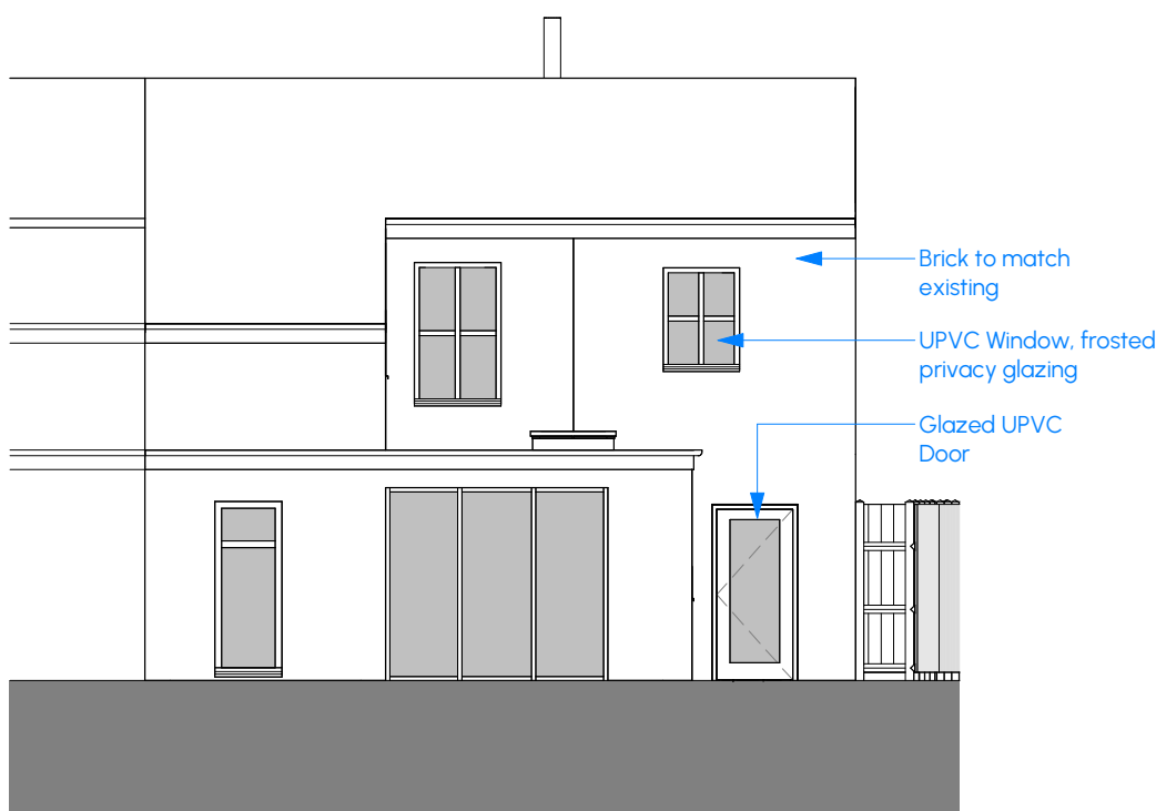
Planning - Proposed Rear Elevation C 1:100
