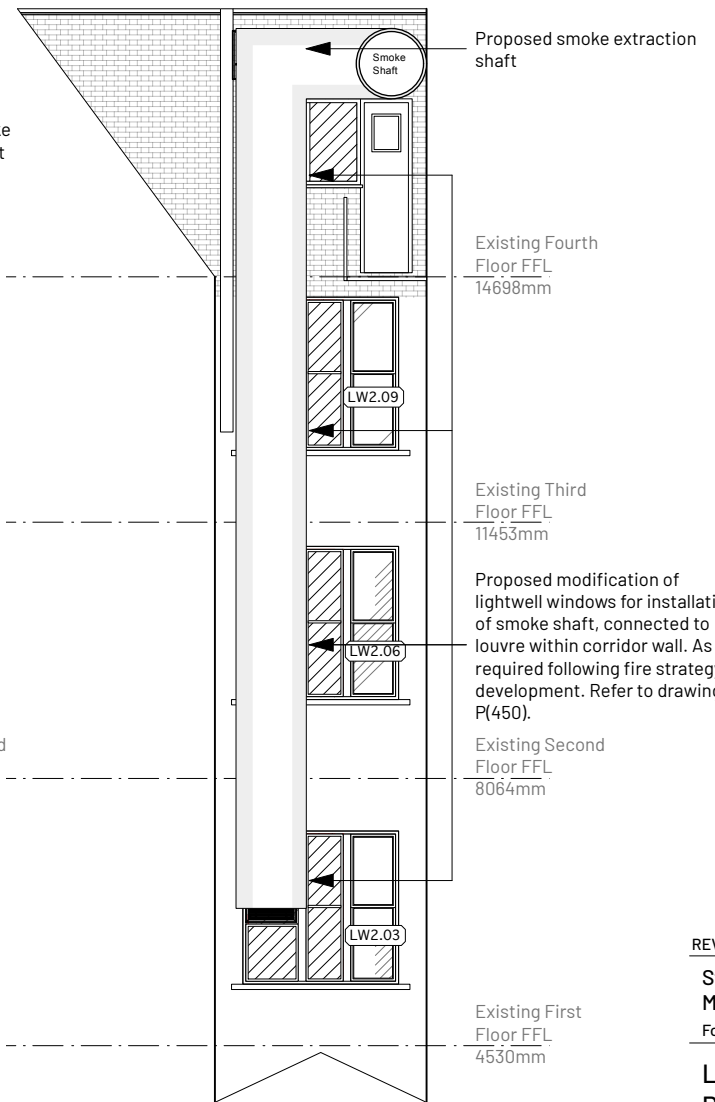
5 Lightwell Elevation DD Scale: 1:100
