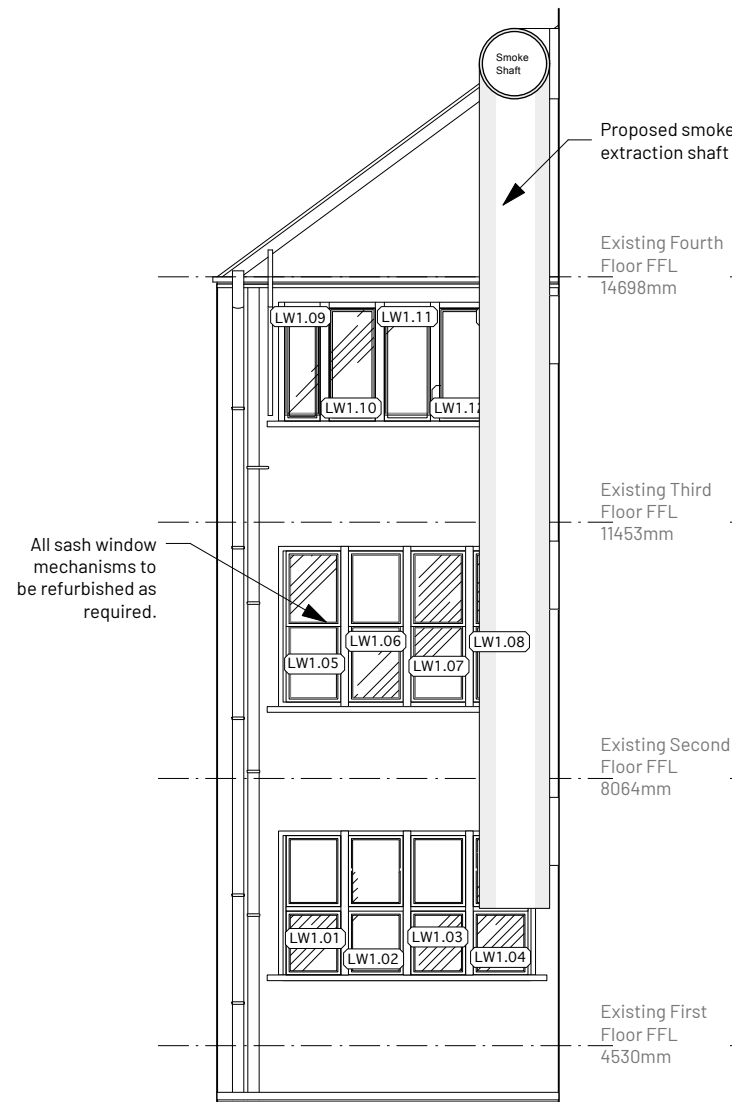
4 Lightwell Elevation CC Scale: 1:100
