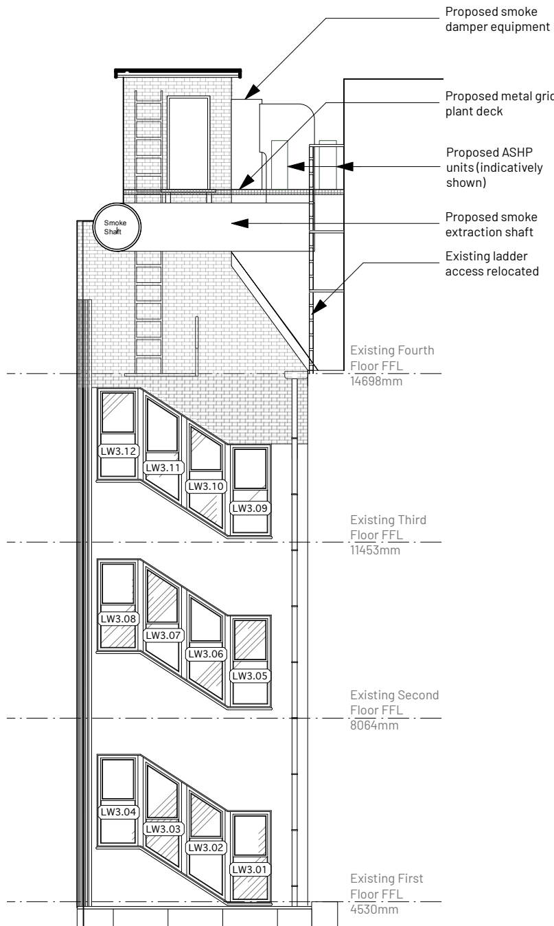
2 Lightwell Elevation AA Scale: 1:100
