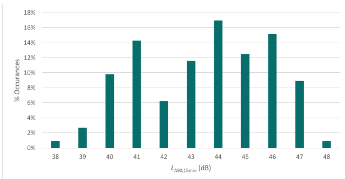
Figure 2: Statistical analysis of background sound pressure levels, daytime
