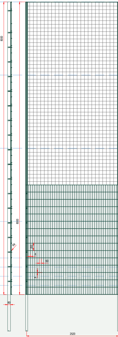
3m site perimeter with new black 100 x 100 ballstop netting installed above, i.e. netting installed from 3.0m to 8.0m high behind goal end next to Islamic Academy. Extended posts are to be powder coated RAL 6005 green to match existing posts.
