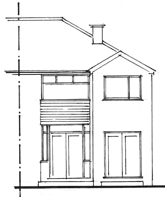
REAR ELEVATION
