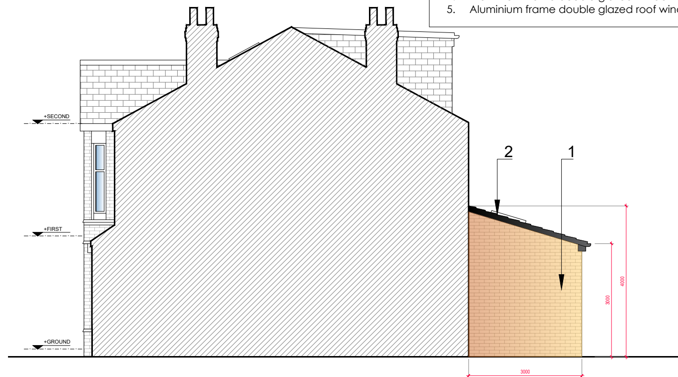
• Proposed Side Elevation (From No 127)
