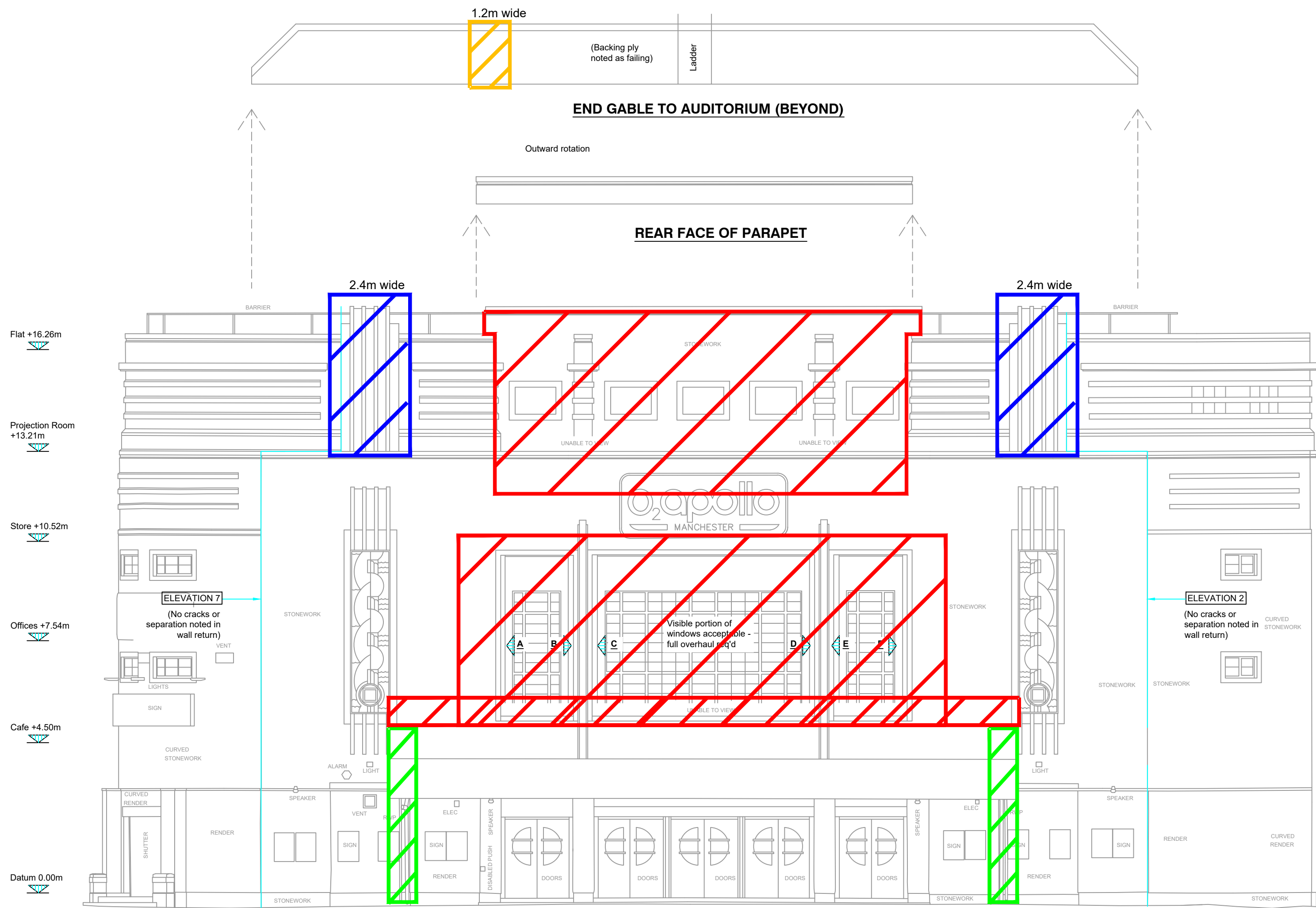
ELEVATION 1 SCALE 1:75
