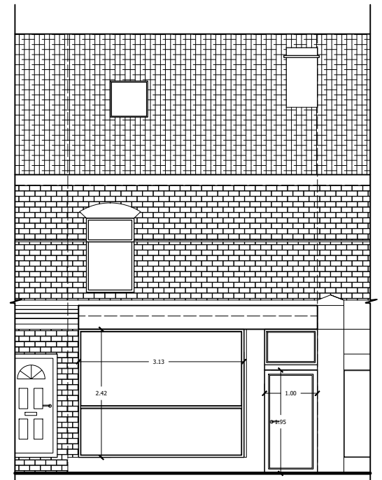
Proposed Front View
