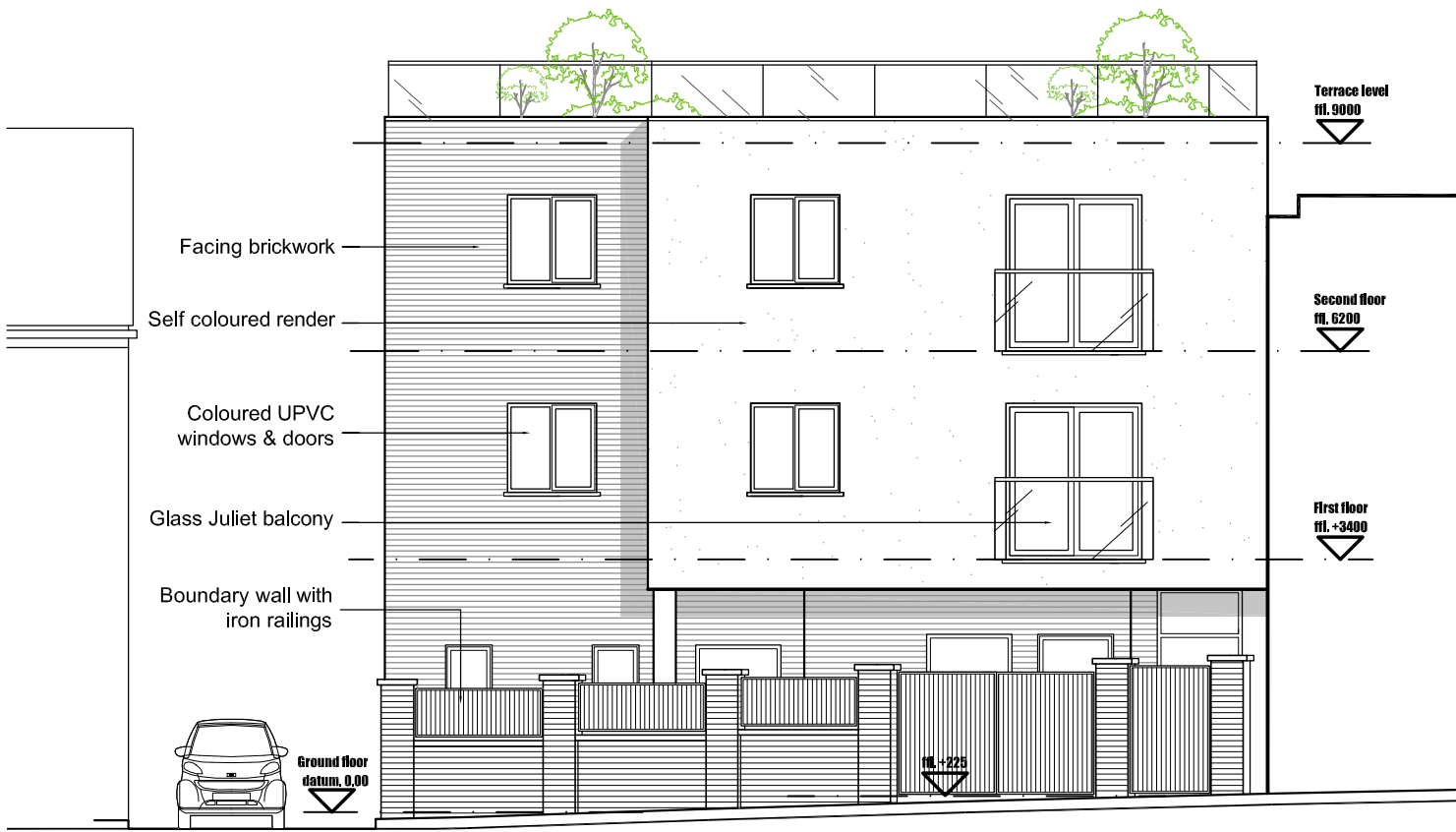
Proposed Rear (North East) Elevation
