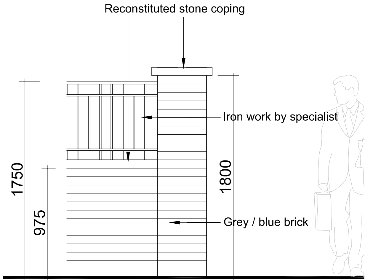
Boundary Wall Detail 1:10
