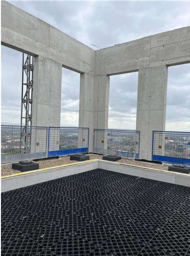
Block 1 Blue Roof Attenuation Crates Photo
