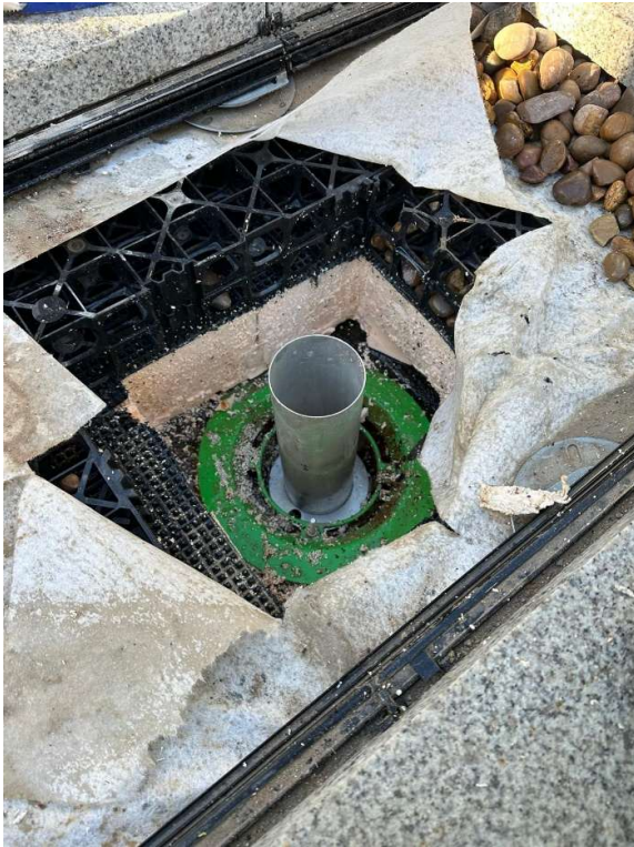
Flow Control Photo – typical roof drainage
