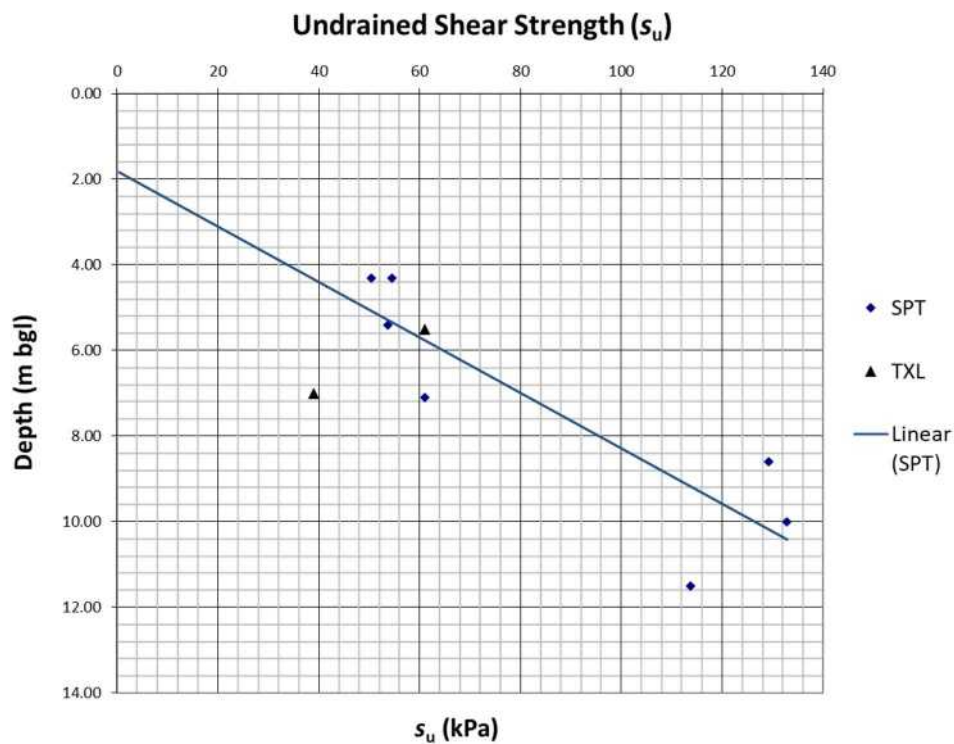
Graph 5-2: Summary of s_u Vs. Depth from In-Situ SPT and TXL Testing.
