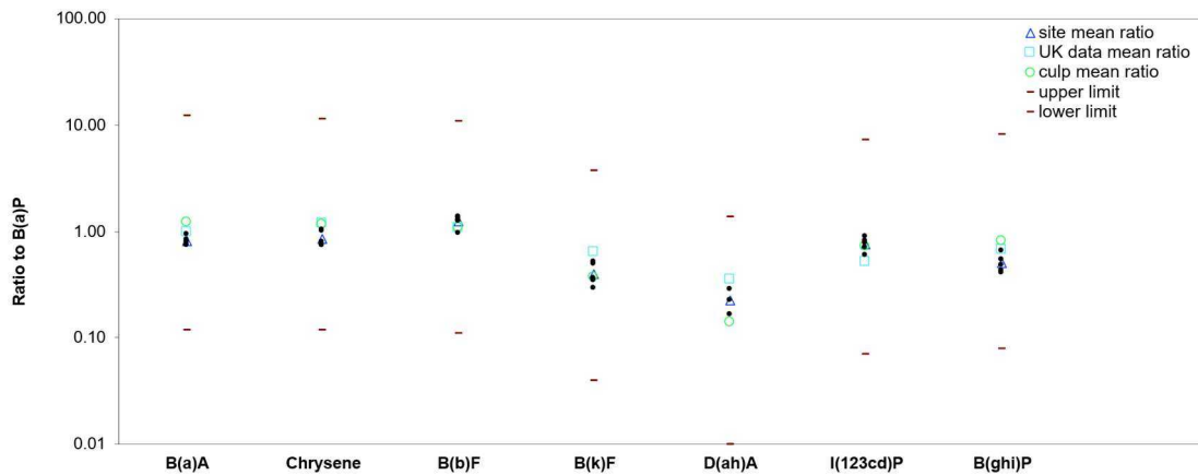
Graph 6-1: The ratio of PAH to B(a)P in soil for all available data at the site based on 8 samples (where values were >LOD to allow the calculation of a ratio).
