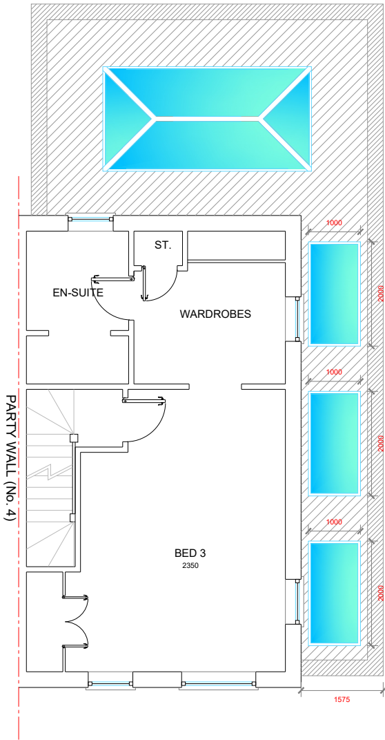
SECOND FLOOR
