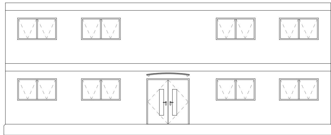
3 Temporary Teaching Building West Elevation 1:100
