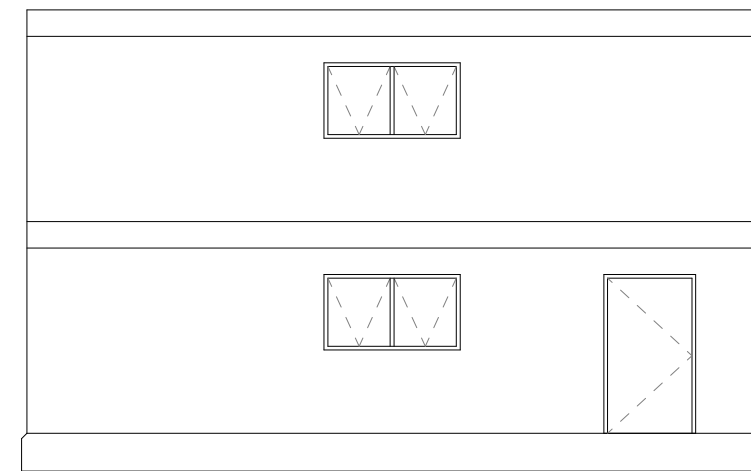
4 Temporary Teaching Building South Elevation 1:100
