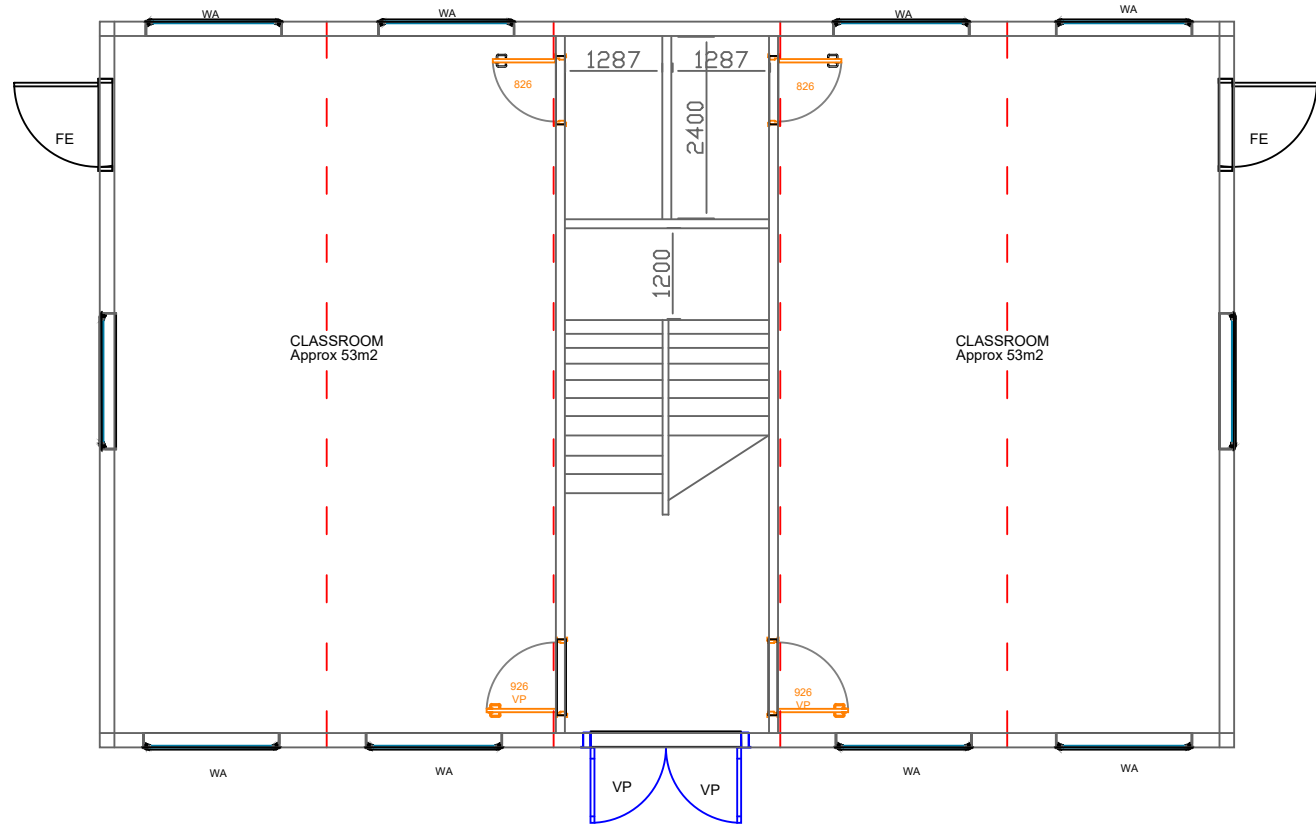
1 Temporary Teaching Building Ground Floor 1:100
