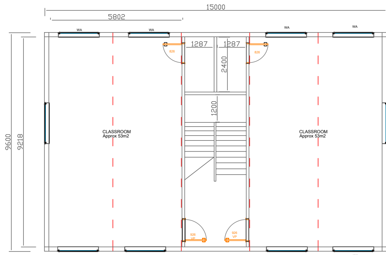
2 Temporary Teaching Building First Floor 1:100
