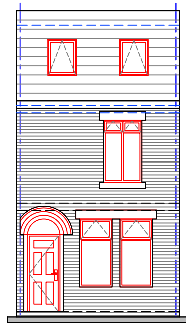
PROPOSED FRONT ELEVATION 1:100
