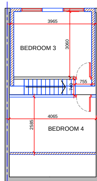
PROPOSED DORMER 1:100
