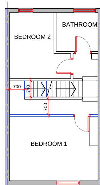
PROPOSED FIRST FLOOR 1:100
