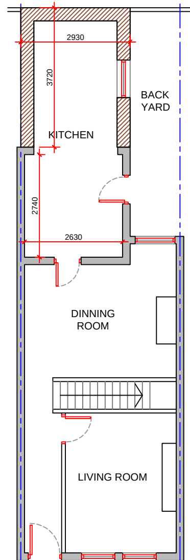
PROPOSED GROUND FLOOR 1:100
