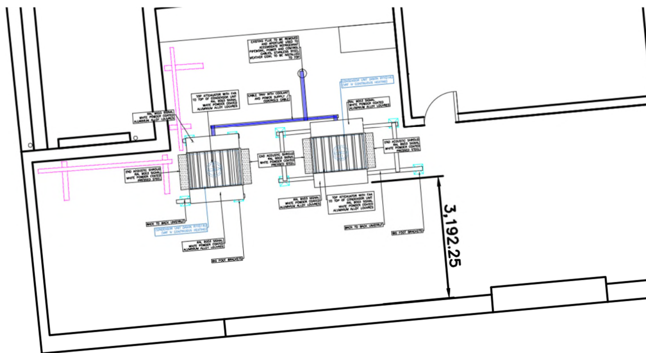
Figure 1 – Partial proposed roof plan showing layout of the units
