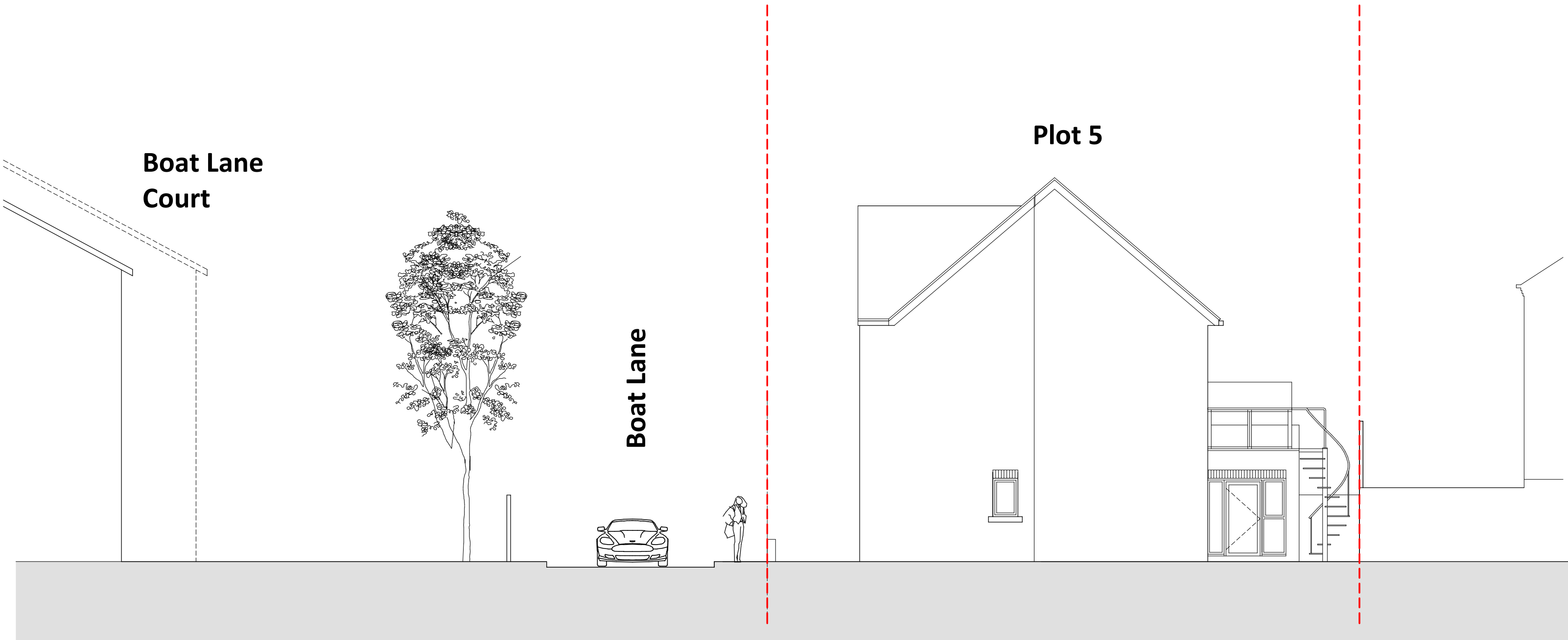
Street Elevation BB - Gable Elevation 1
