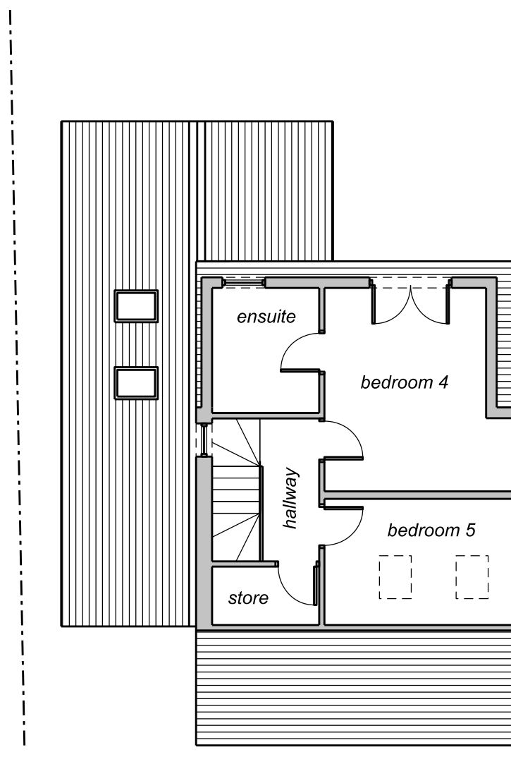
Loft Floor Plan
