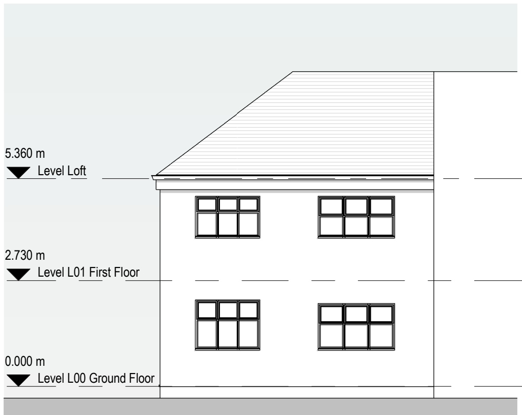
3 Existing North Elevation 1 : 100
