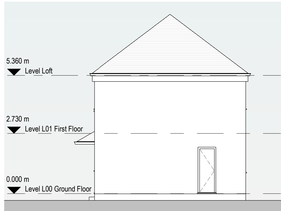
2 Existing EastX Elevation 1 : 100
