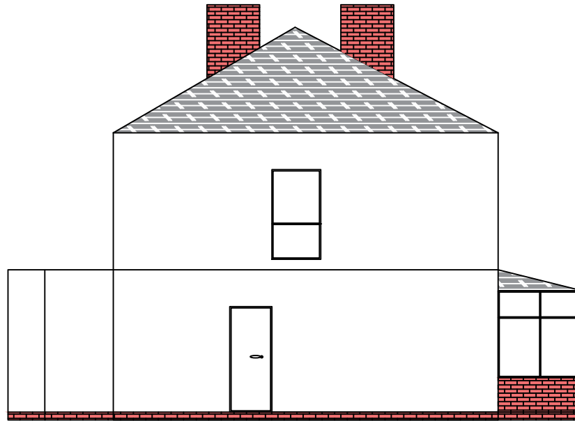
Existing side elevation Scale 1:100 on A4
