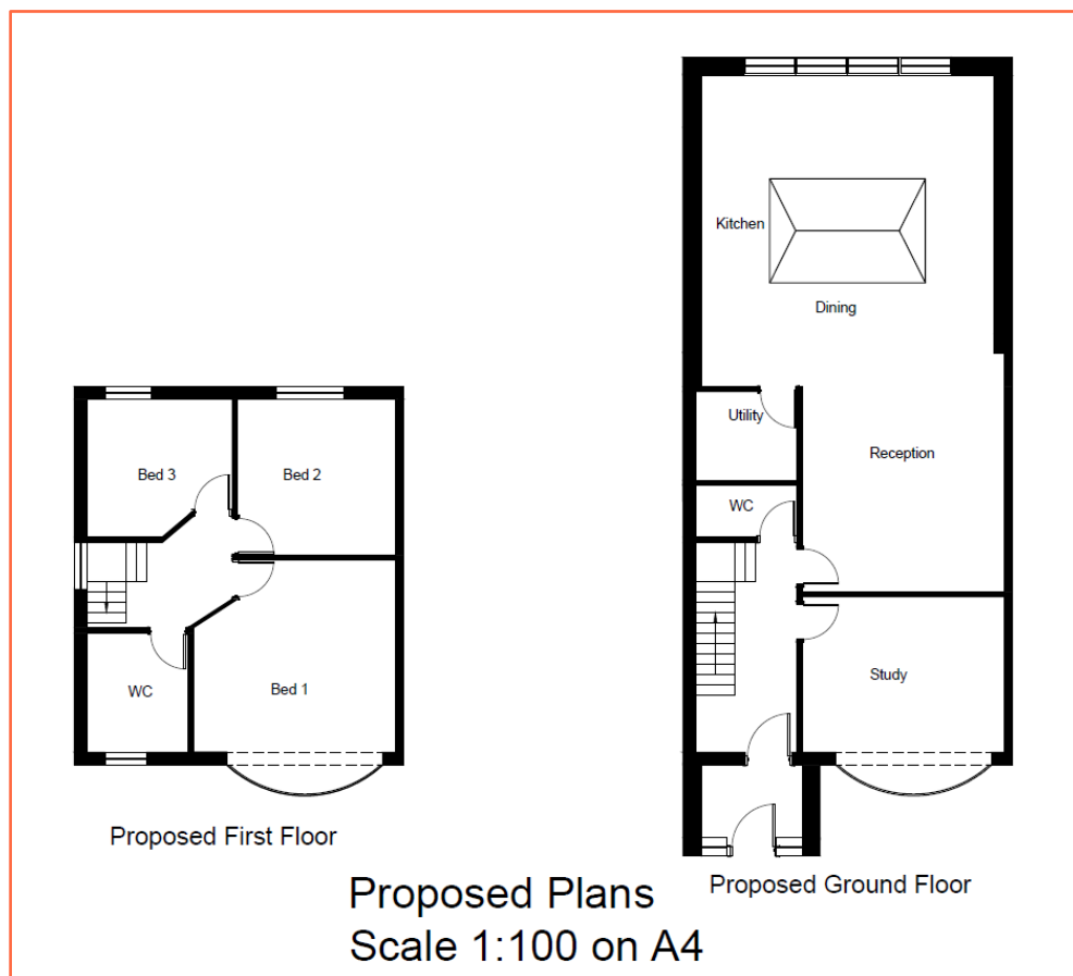
Figure 5: Proposed ground and first floor plan (Source: Applicant)
