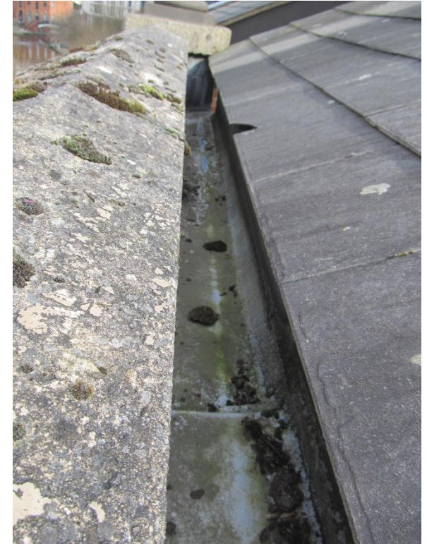
3. Lead lined back parapet gutter
