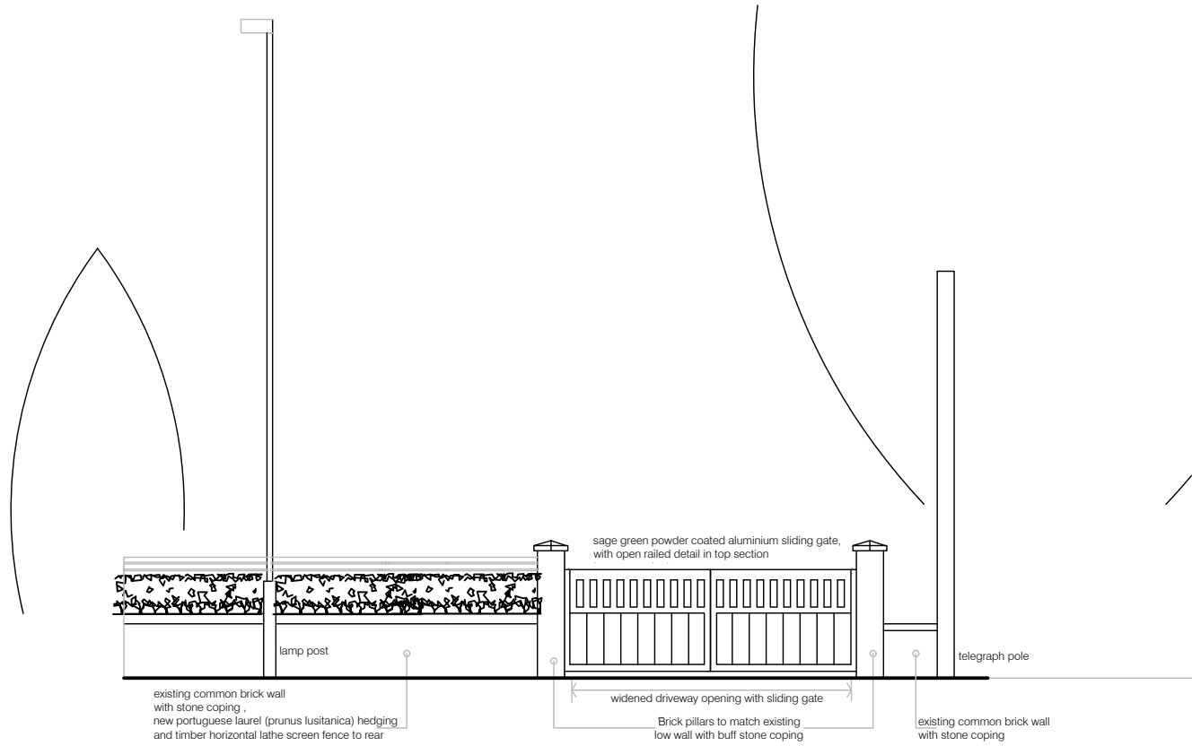
PROPOSED STREET ELEVATION
