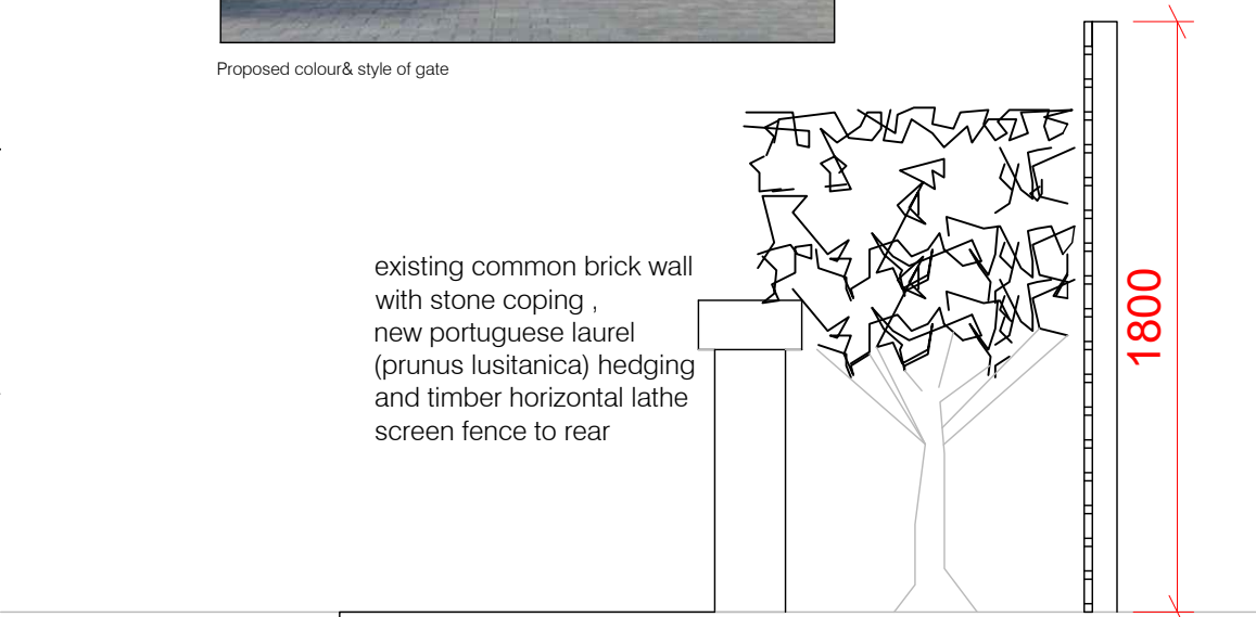
SECTION THRO FRONT WALL 1:25
