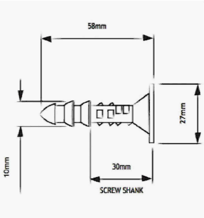
Delta Qwikseal plug fixings
