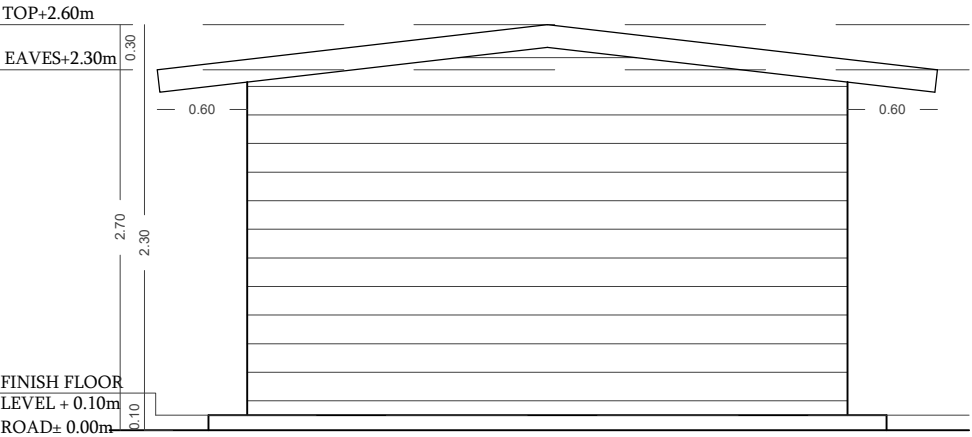
REAR SIDE ELEVATION FACES SOUTH SCALE=1:50
