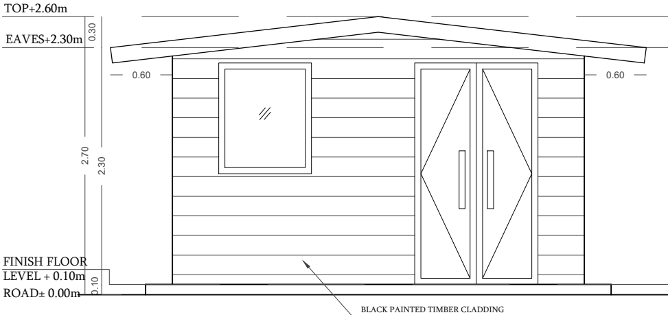
FRONT ELEVATION FACES NORTH SCALE=1:50
