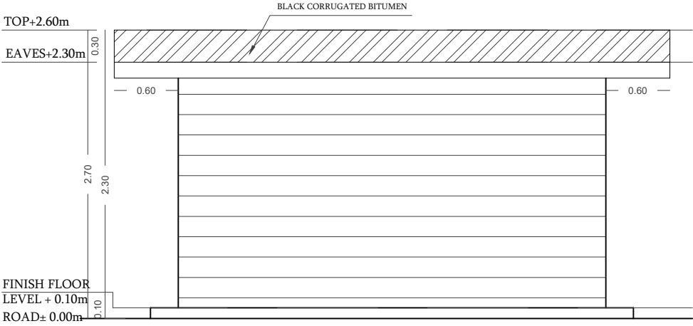
LEFT SIDE FACES WEST SCALE=1:50
