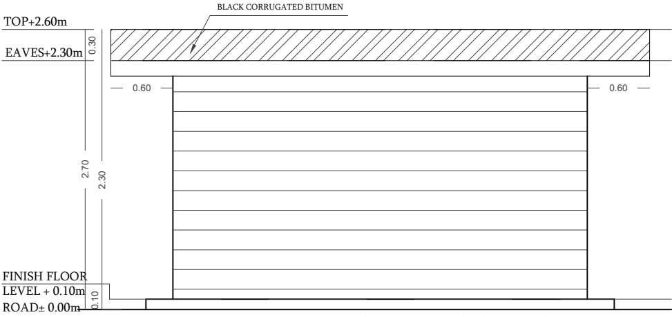
RIGHT SIDE ELEVATION FACES EAST SCALE=1:50
