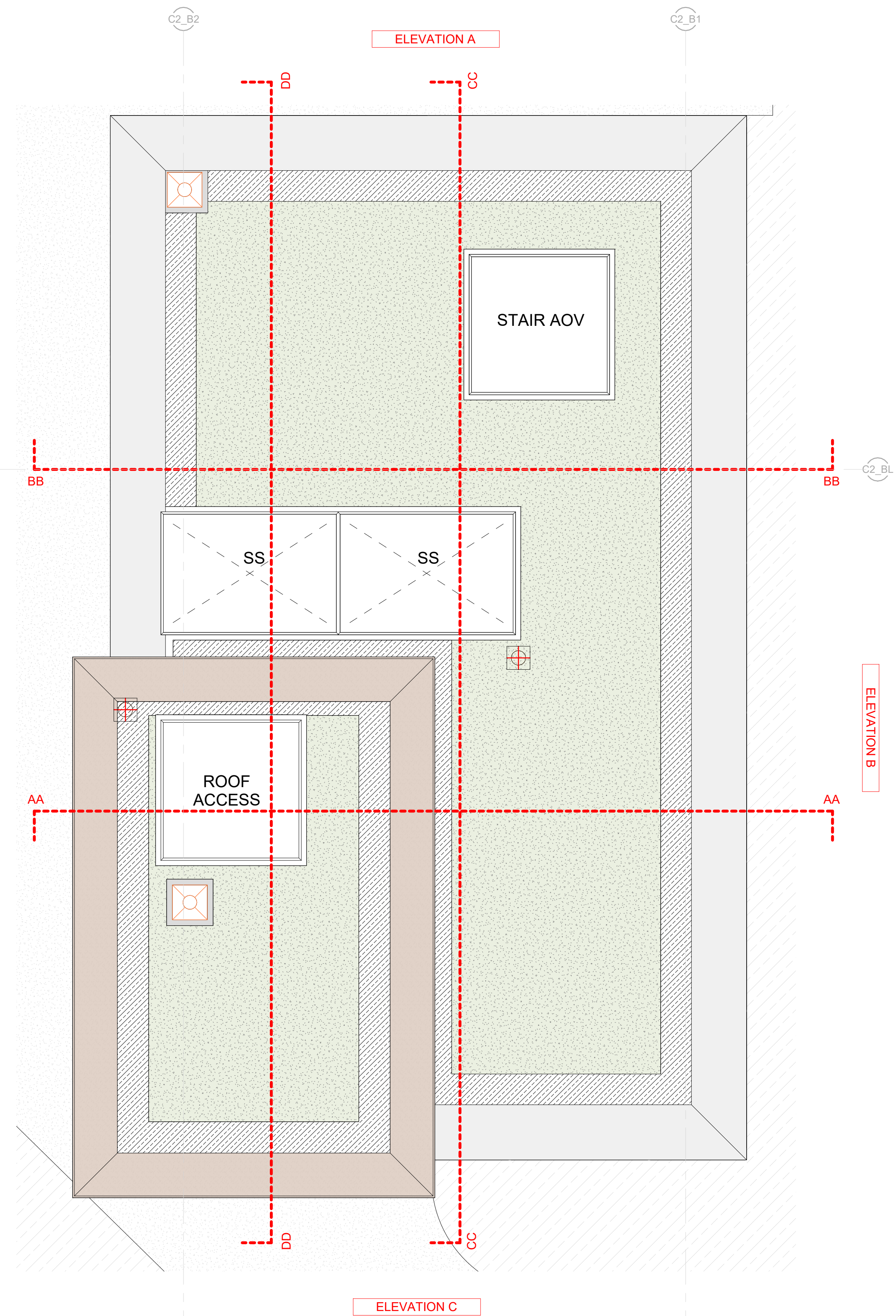
2 G251_C2_Core Pop Up_Roof Plan 1 1:25
