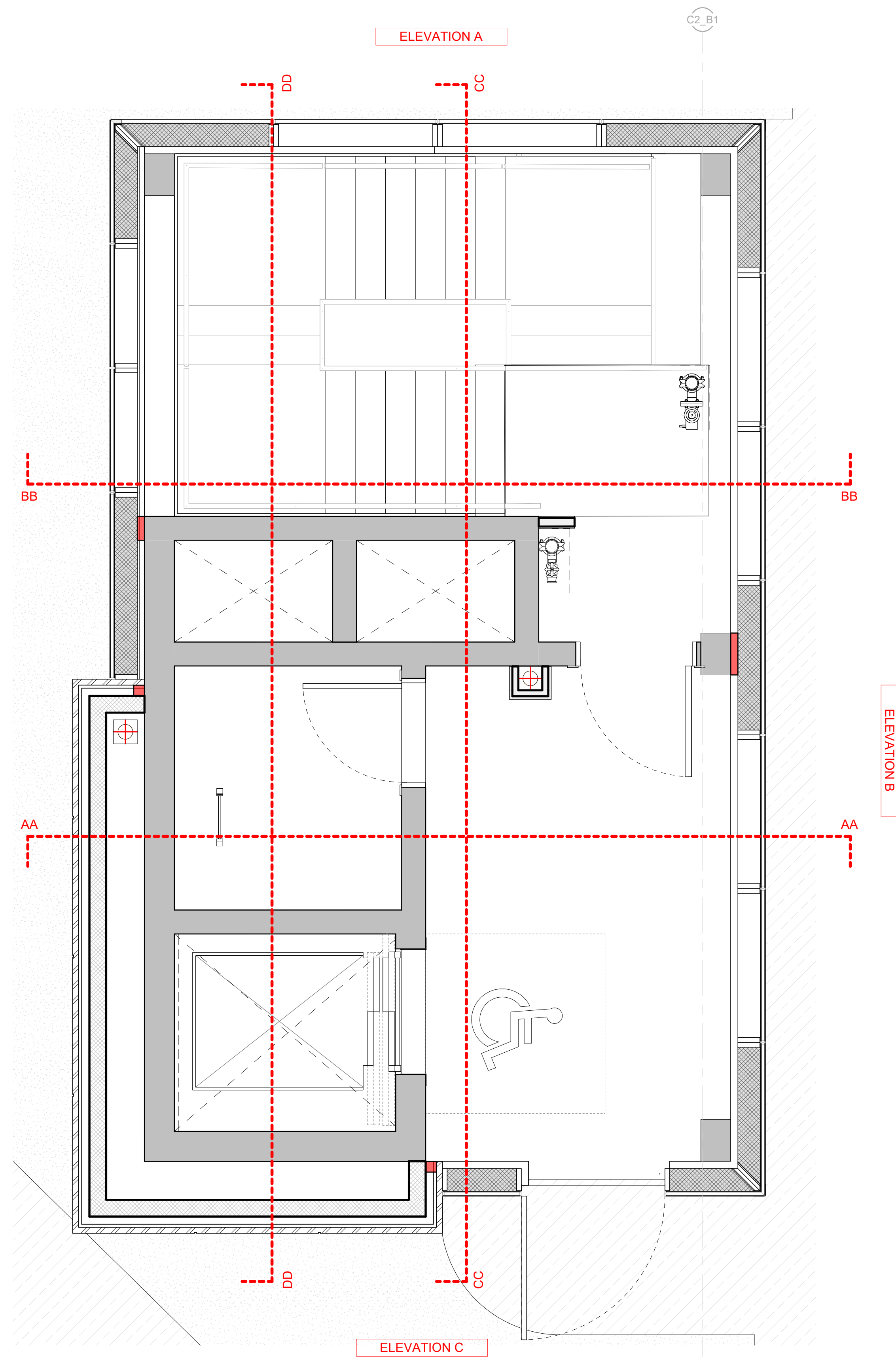
1 G251_C2_Core Pop Up_Plan 1 1:25
