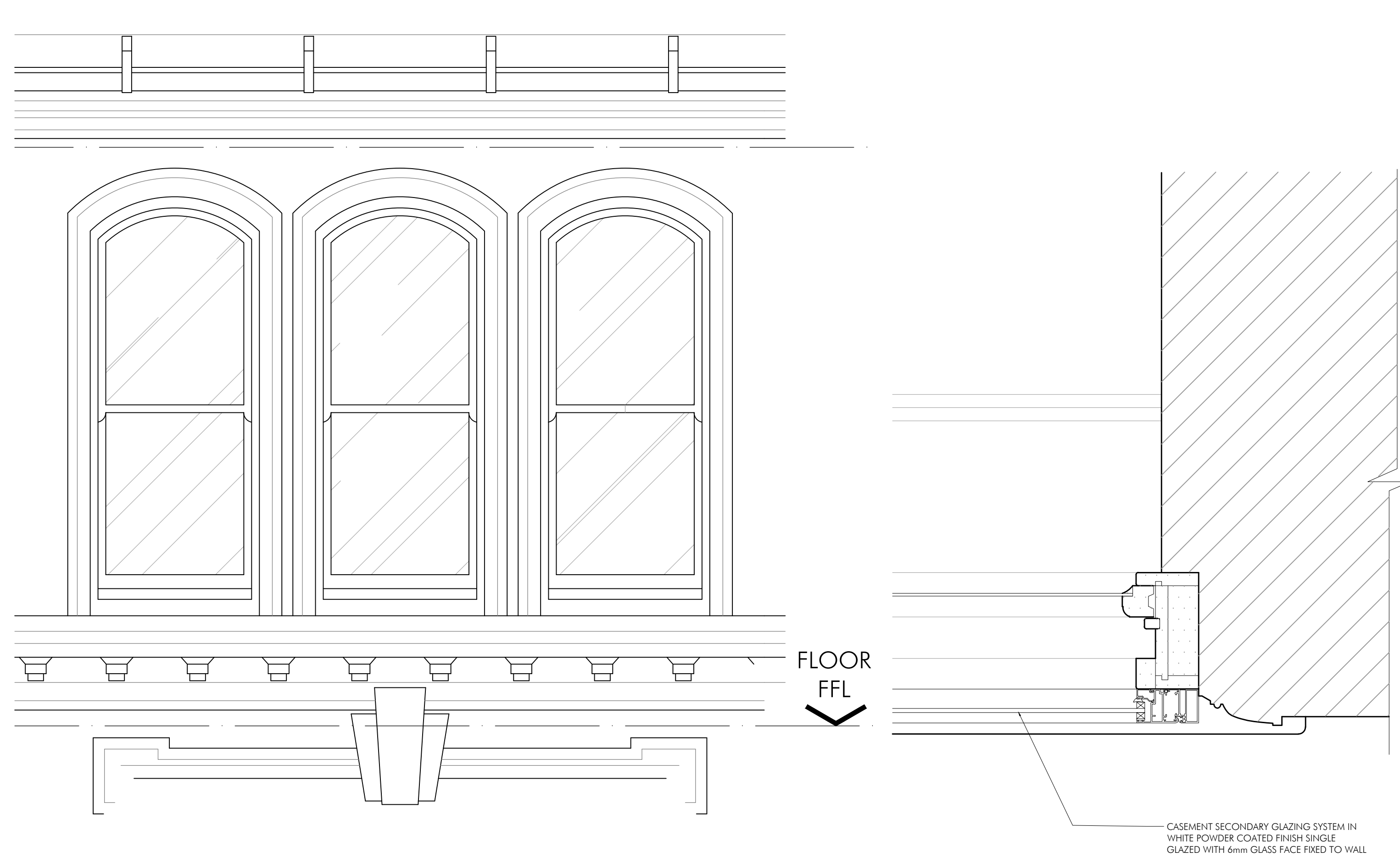
TYPICAL THIRD FLOOR FRONT EXTERNAL WINDOW ELEVATION SCALE 1:20
