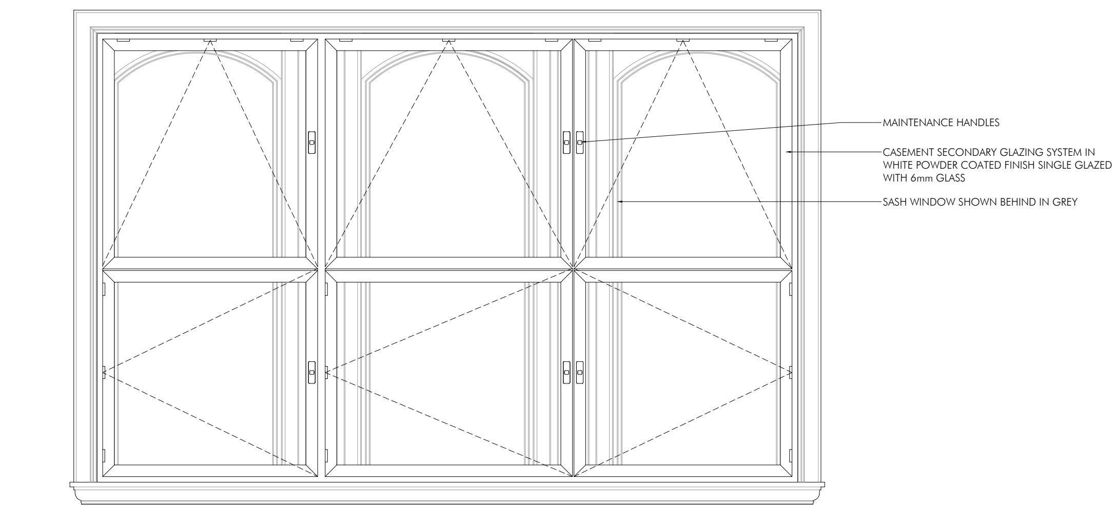
TYPICAL THIRD FLOOR FRONT INTERNAL WINDOW ELEVATION SCALE 1:20
