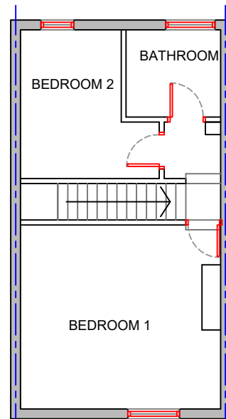
PROPOSED FIRST FLOOR
