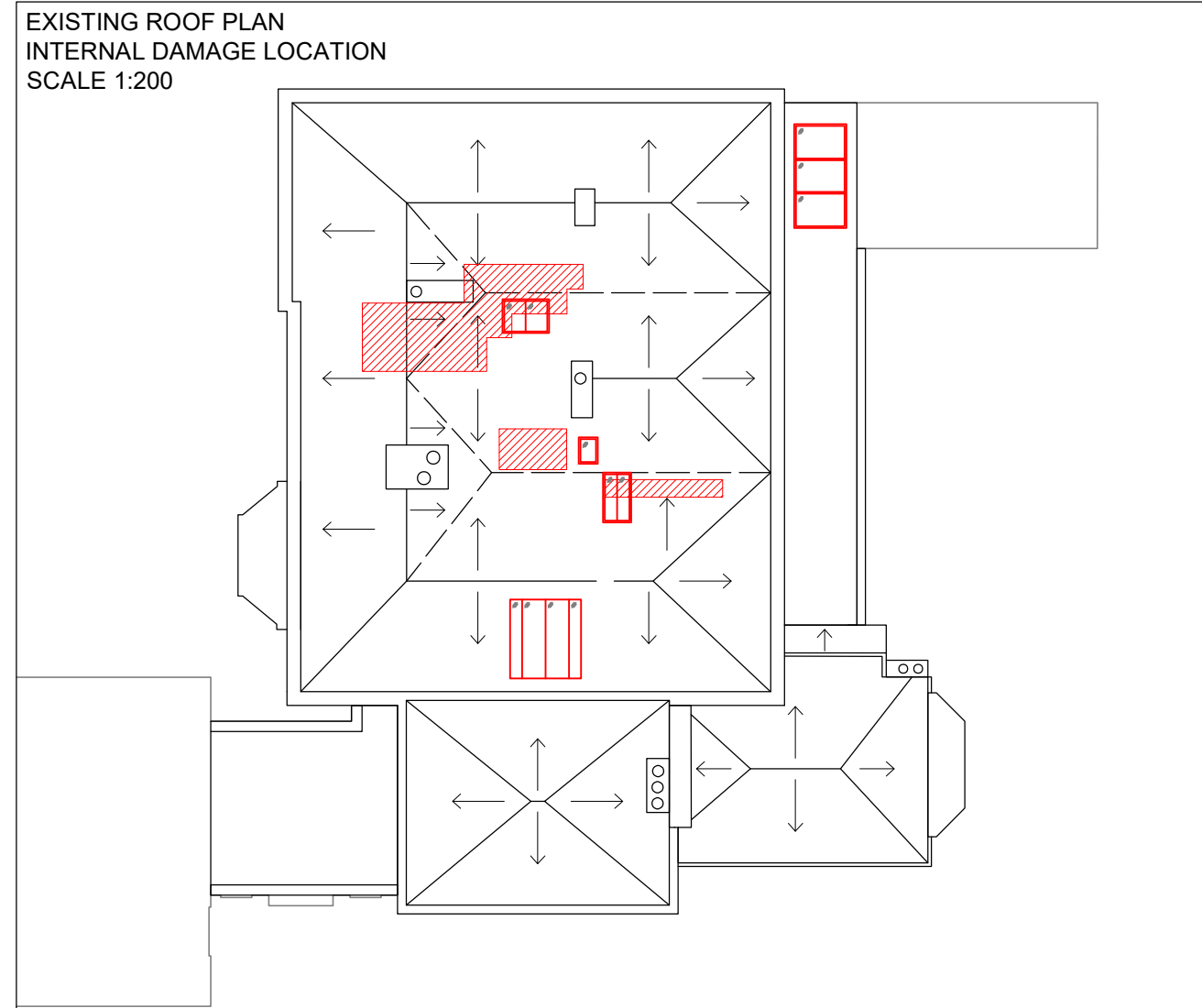
THE INFORMATION ON THIS DRAWING RELATES TO THE DETAIL OF THE EXISTING BUILDINGS IS INDICATIVE ONLY, AS DETAILED MEASURED SURVEYS ARE YET TO BE COMPLETED. THE LOCATION AND DIMENSIONS OF ALL EXISTING EXTERNAL AND INTERNAL BUILDING ELEMENTS SHOULD BE VERIFIED ON SITE. THIS DRAWING SHOULD BE READ IN CONJUNCTION WITH THE ARCHITECT'S DRAWINGS, SPECIFICATION AND SCHEDULES, AND THOSE PROVIDED BY THE OTHER CONSULTANTS. GENERAL ALL PROFILES ARE PROVISIONAL, SUBJECT TO FURTHER INSPECTION ONCE SUITABLE ACCESS PROVISIONS HAVE BEEN PROVIDED, WHERE PROFILES ARE TO BE MATCHED EXACTLY TO AN EXISTING PROFILE. DRAWN PROFILES ARE INDICATIVE AND FOR INFORMATION ONLY. THE CONTRACTOR SHALL ALLOW FOR THE PROFILES OF THE EXISTING AND PROVIDE FABRICATION DRAWINGS AND SAMPLES, AS SPECIFIED, PRIOR TO MANUFACTURE. SLATE THE ROOF PITCHES ARE TO BE RE-CLIMBED, COMPLETE RAFTERS TO SARKING AND RAFTERS AS REQUIRED TO BE REPLACED BY AN APPROVED PROJECTOR GROUP/SHIELD BREATHING VAPOUR PERMEABLE MEMBRANE OR EQUIVALENT (TO BE AGREED). EXISTING SLATES ARE TO BE CAREFULLY REMOVED AND STORED FOR RE-INSTALLMENT. THE CONTRACTOR IS TO ALLOW FOR SPLITTING REMOVED SLATES BEFORE RE-COVERING AND ALLOW FOR RE-HOLING / DRESSING AS NECESSARY. ALL SLATES SHOULD RING WHEN STRUCK, AND ALL CRACKED, DRAFT, SORT OR PITCHED SLATES ARE TO BE REJECTED. HEAD LATHES ARE TO BE REMOVED FROM THE HEAD OF THE SLATE. ANY SHORTFALL IN REQUIRED RE-COVERING QUANTITIES ARE TO BE CONFIRMED WITH THE CA PRIOR TO REPLACING, REPLACEMENT / SHORTFALL SLATES ARE TO BE PROCURED FROM SUITABLE UK QUARRIES IN ACCORDANCE WITH THE RELEVANT BUILDING REQUIREMENTS PRESCRIBED WITHIN BS. NO SOUND RE-CONFORMANCE SLATES ARE TO MATCH EXISTING IN TYPE, SIZE, THICKNESS, COLOUR AND TEXTURE. SAMPLES ARE TO BE PROVIDED AND BE APPROVED BY THE CA PRIOR TO RE-INSTALLMENT. LEAD ALL NEW LEADWORK AND LEAD DETAILS ARE TO BE AS GUIDANCE FOR STATUTORY DESIGNATED HISTORIC BUILDINGS. ALL LEAD SHEET IS TO BE TO BS EN 12898 AND INSTALLED IN ACCORDANCE WITH BS 6915 AND THE LATEST EDITION OF LEAD SHEET TRAINING ACQUAINTANCE (LSTA) ROLLED-LEAD SHEET, THE COMPLETE MANUAL. ALL LEADWORK IS TO BE CARRIED OUT BY A PERSON WITH PROVEN SKILLS IN THE APPLICATION OF LEAD COVERINGS AND EMPLOYED BY A MEMBER OF THE LEAD CONTRACTORS' ASSOCIATION. ON COMPLETION THE LEAD WORK SHALL BE REGISTERED UNDER THE LCA MEMBERS' 25 YEAR GUARANTEE SCHEME. LEAD AND OTHER MATERIALS REPLACE MEMBRANE TO BE FITTED ABOVE SARKING/BAR / RAFTERS AS SPECIFICATION SECTION H62. ALL LEAD WORK TO BE LAID ON NEW BUILDING PAPER CONFORMING TO BS 1521 CLASS 1. LEAD SHOULD ONLY BE LAYED ON DRY SUBSTRATE AND UNDERLAY TO AVOID CORROSION. NEUTRAL COLE POLYURETHANE IS TO BE USED TO SEAL THE JOINTS BETWEEN LEAD SHEET AND OTHER BUILDING MATERIALS. METALWORK FIT HAND ACCESS POINTS AT BASE OF ALL DOWNPIPES. OVERHAUL ALL EXISTING RETAINED GUTTERS, INCLUDING FULL RE-CALLING OF ALL JOINTS. FLUSH FLIP FLIP PREPARE AND PAINT TO MATCH EXISTING, ALL IN ACCORDANCE WITH MANUFACTURERS RECOMMENDATIONS, INCLUDING MANUFACTURERS RECOMMENDATION OF EXISTING METALWORK PRIOR TO COATING. ROOFLIGHTS EXISTING CORRUGATED, MODERN ROOF LIGHT (RPL) TO BE REMOVED AND REVEAL. PREPARED IN READINESS TO RECEIVE NEW UNIT IN ACCORDANCE WITH SPECIFICATION SECTION L10. EXISTING SINGLE PANE VIBROD GLAZED ROOF LIGHTS (RL2 THRU 5) ARE TO BE RETAINED AND SURVEYED ONCE SUITABLE ACCESS PROVISIONS PROVIDED. ALLOW FOR RE-DRESSING EXISTING GLAZ FLASHING IN ACCORDANCE WITH THE RELEVANT BUILDING REQUIREMENTS PRESCRIBED WITHIN BS. NO SOUND RE-CONFORMANCE GLAZING REPLACEMENT PUTTY BE REQUIRED. UNDERTAKE REMEDIAL WORKS IN ACCORDANCE WITH SPECIFICATION SECTIONS L10 AND L40. NOTE: SHOULD REPLACEMENT ROOF LIGHTS BE REQUIRED POST INSPECTION THIS WILL BE INSTRUCTED BY FORMAL CONTRACT INSTRUCTION FROM PROVISIONAL SUMS AS THE DIRECTION OF THE CA. EXISTING SERVICES REMOVE ALL EXISTING, REDUNDANT SERVICES AND ASSOCIATED FIXINGS AFTER INVESTIGATION ON SITE TO DETERMINE PURPOSE, MAKE GOOD ACONARY AFTER REMOVAL.
