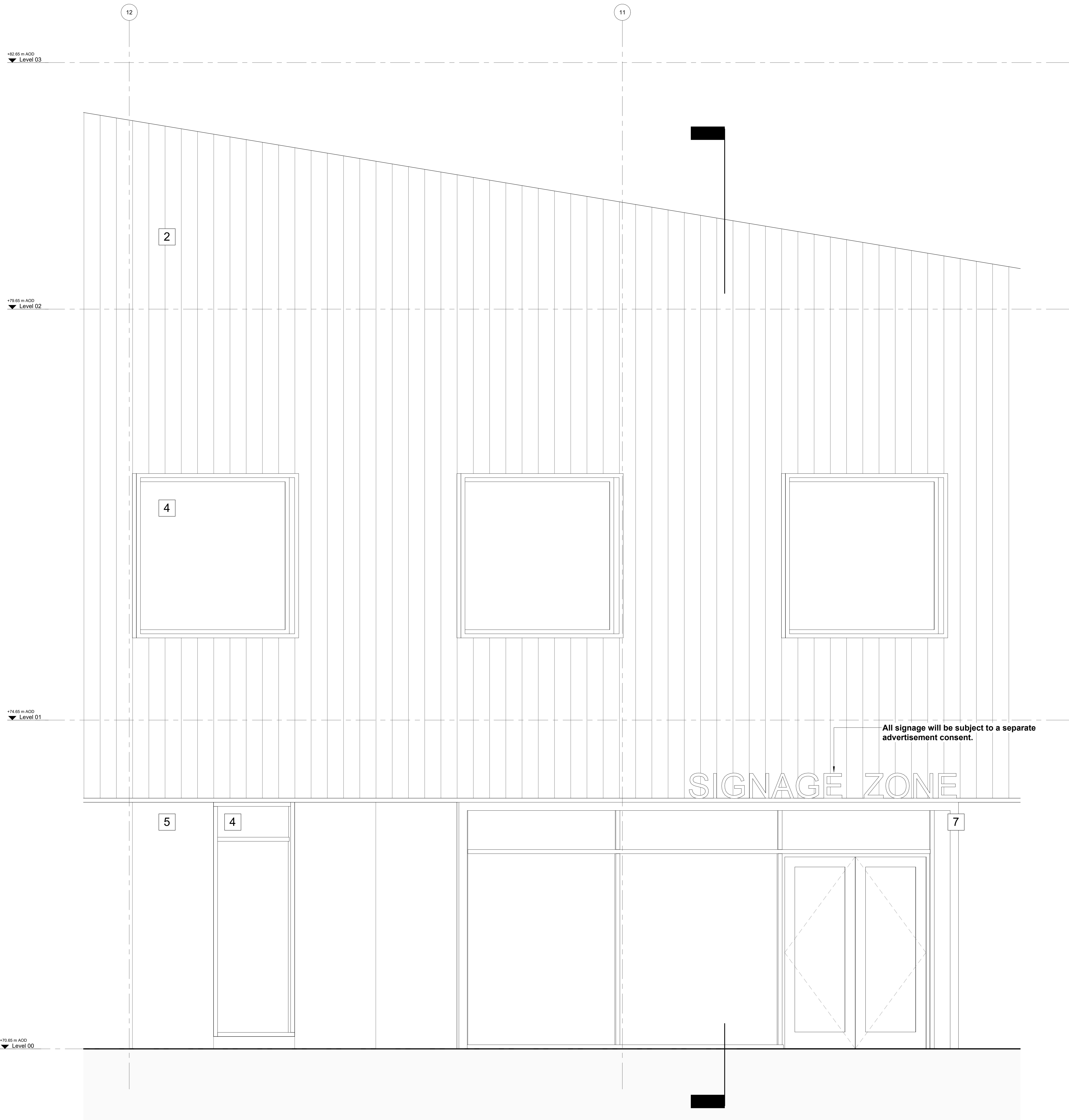
2 Typical Elevation - Through Window and Curtain Walling 1 : 20
