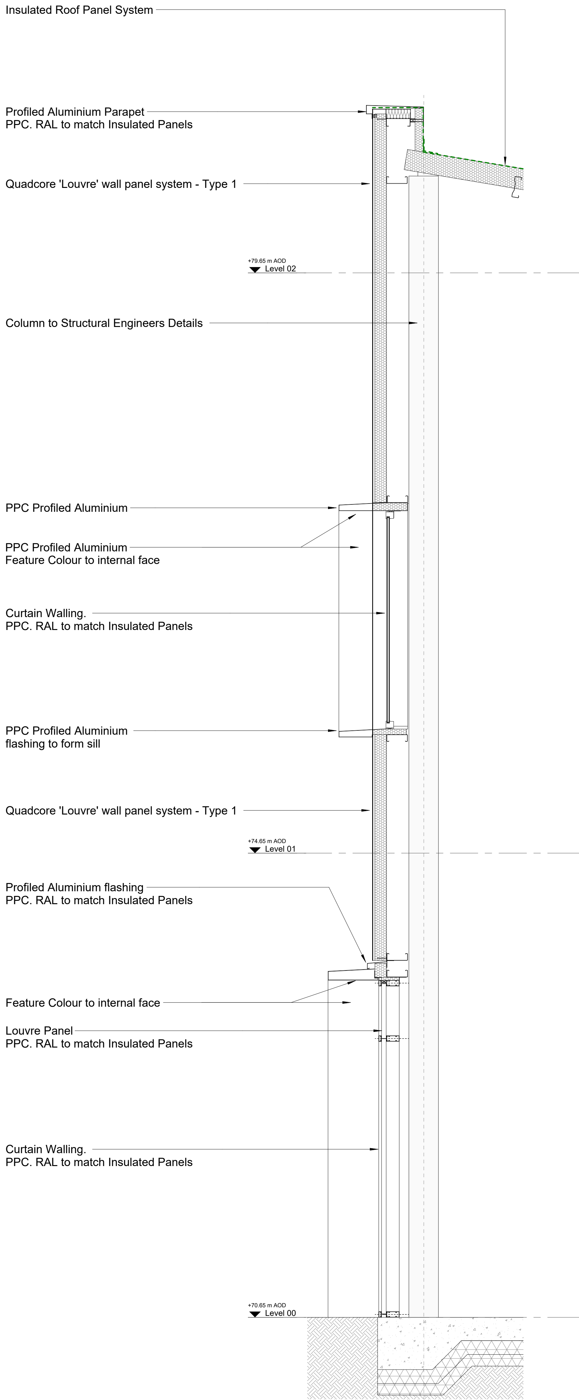
1 Typical Strip Section - Through Window and Curtain Walling 1 : 20
