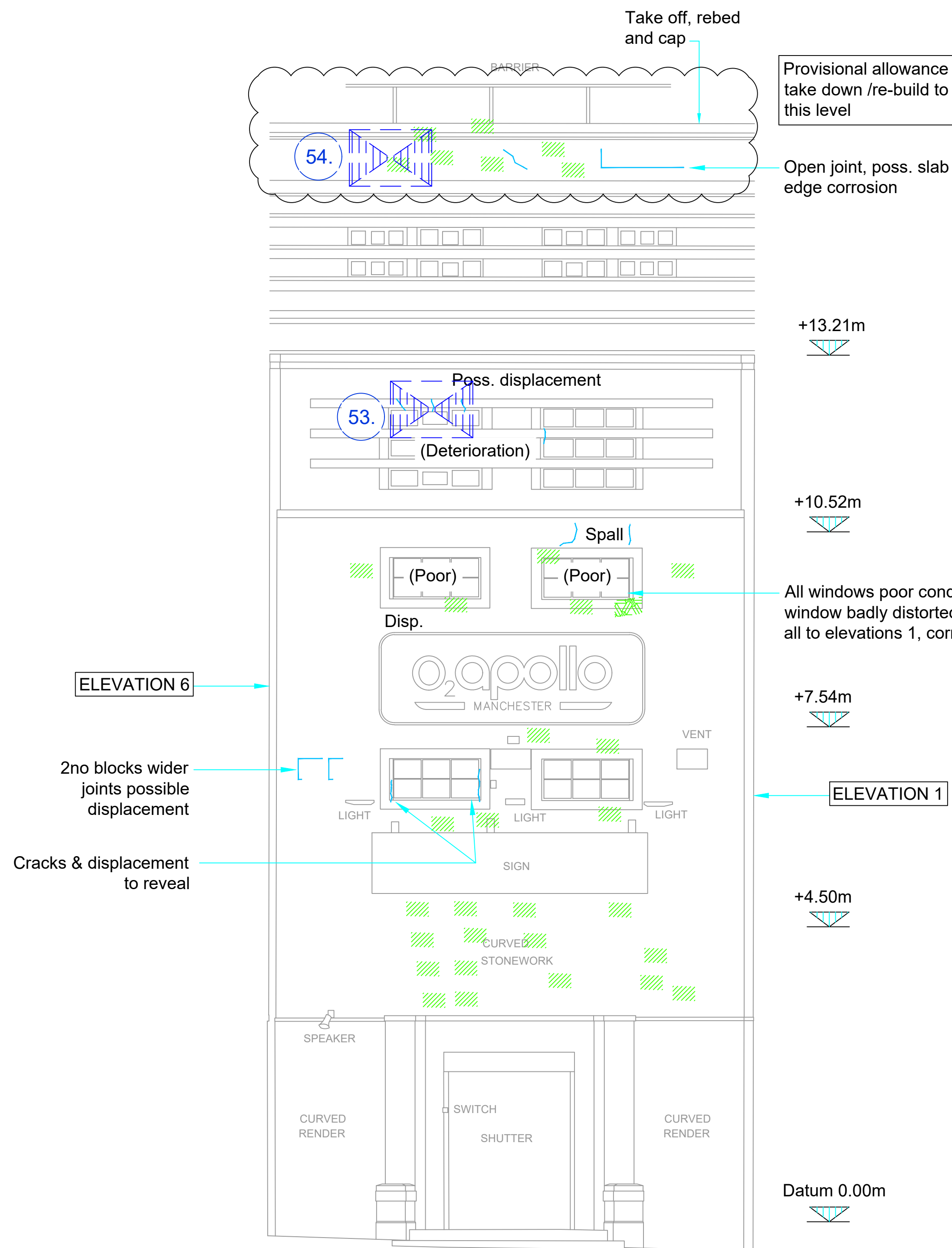
ELEVATION 7 SCALE 1:75
