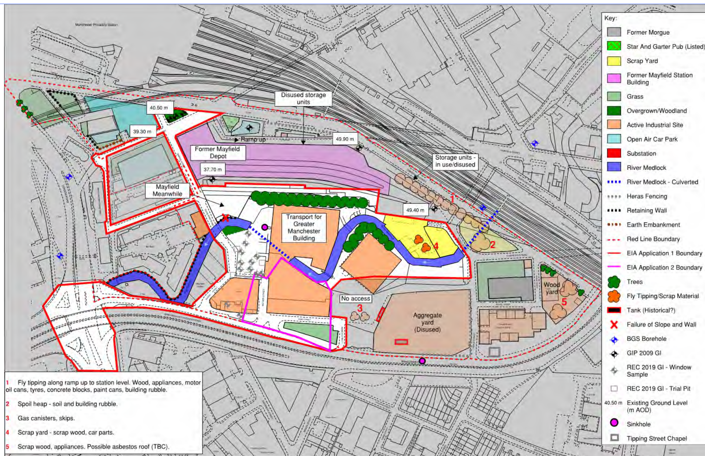
Figure: 10.1 Title: Site Constraints Plan Project: Mayfield Phase 1 Date: September 2019 Scale: NTS
