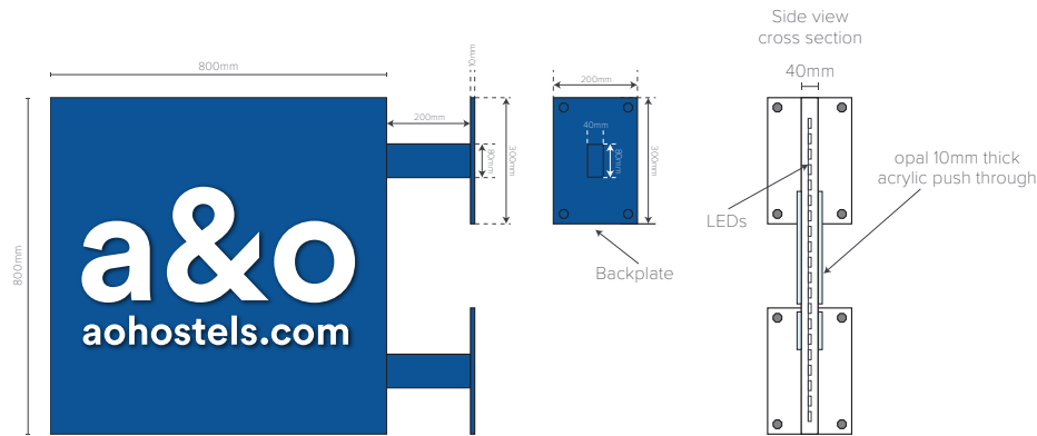
Existing layout
