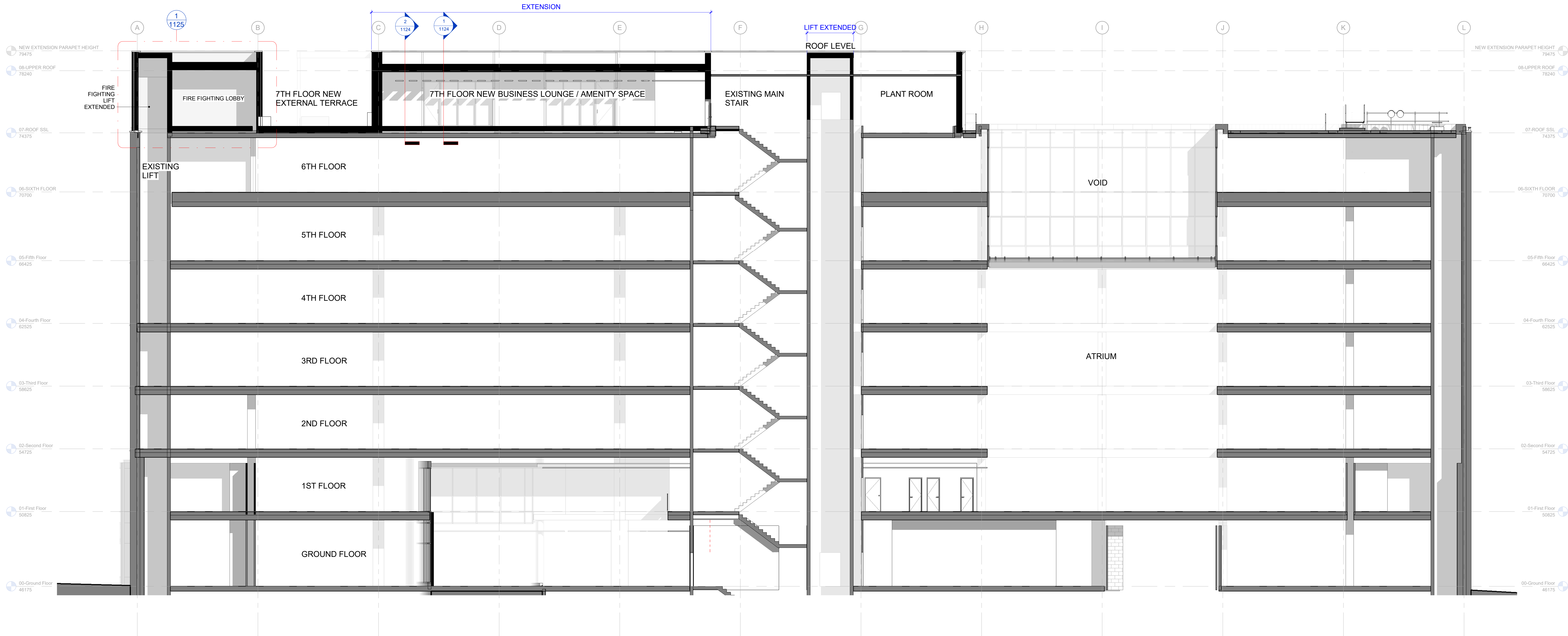
1 PROPOSED SECTION A-A 1 : 100
