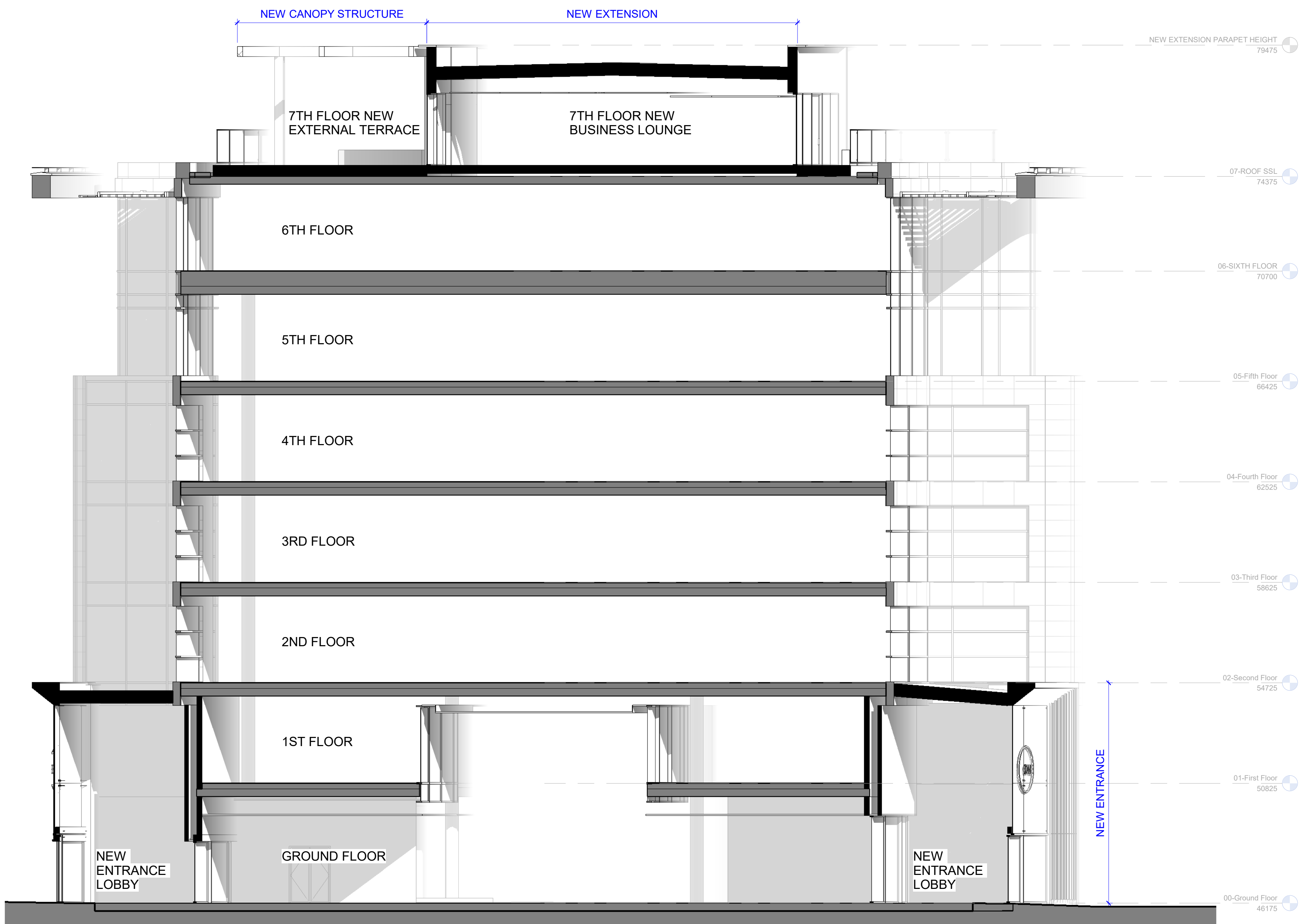
2 PROPOSED SECTION B-B 1 : 100
