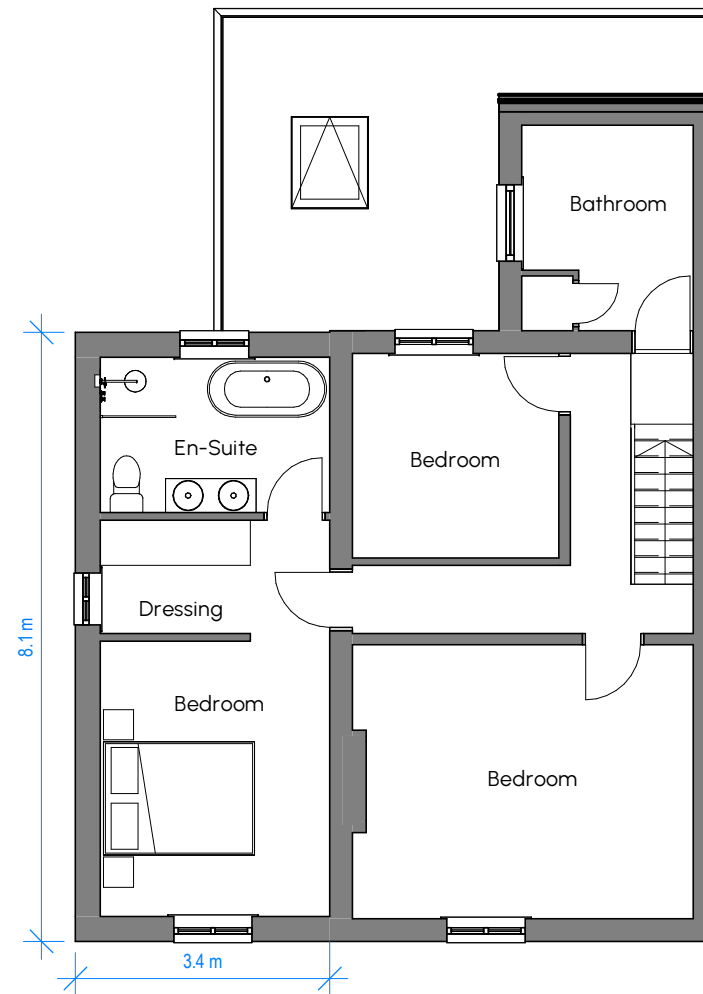
Planning - Proposed First Floor Plan 1 : 100
