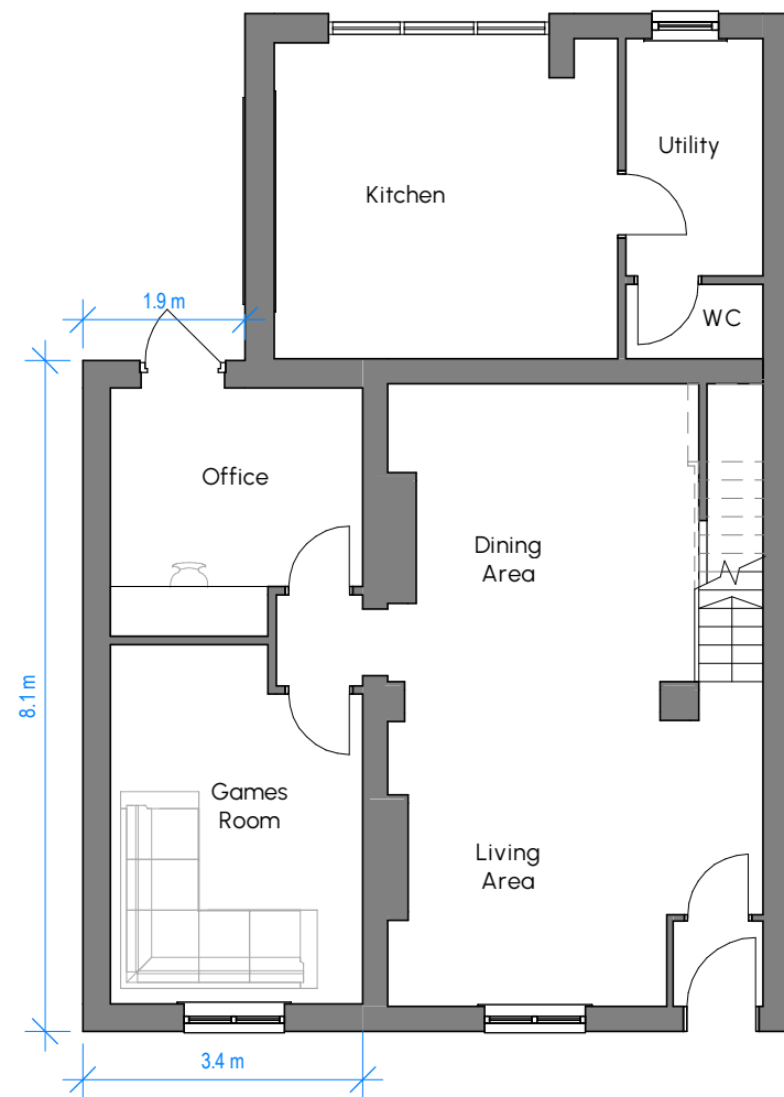
Planning - Proposed Ground Floor Plan 1 : 100
