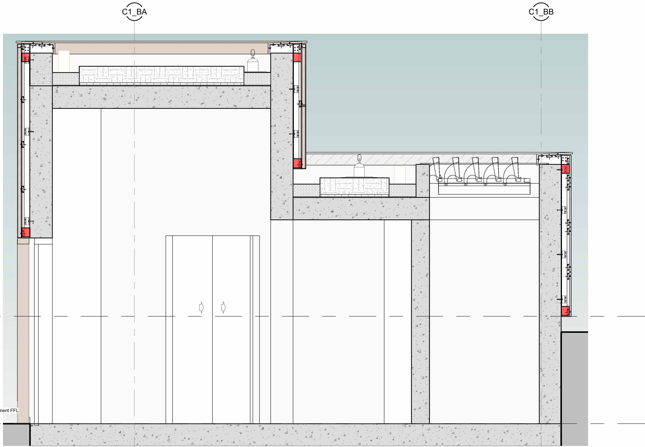
3 G251_C1_Core Pop Up_SE_CC 1 1 : 25
