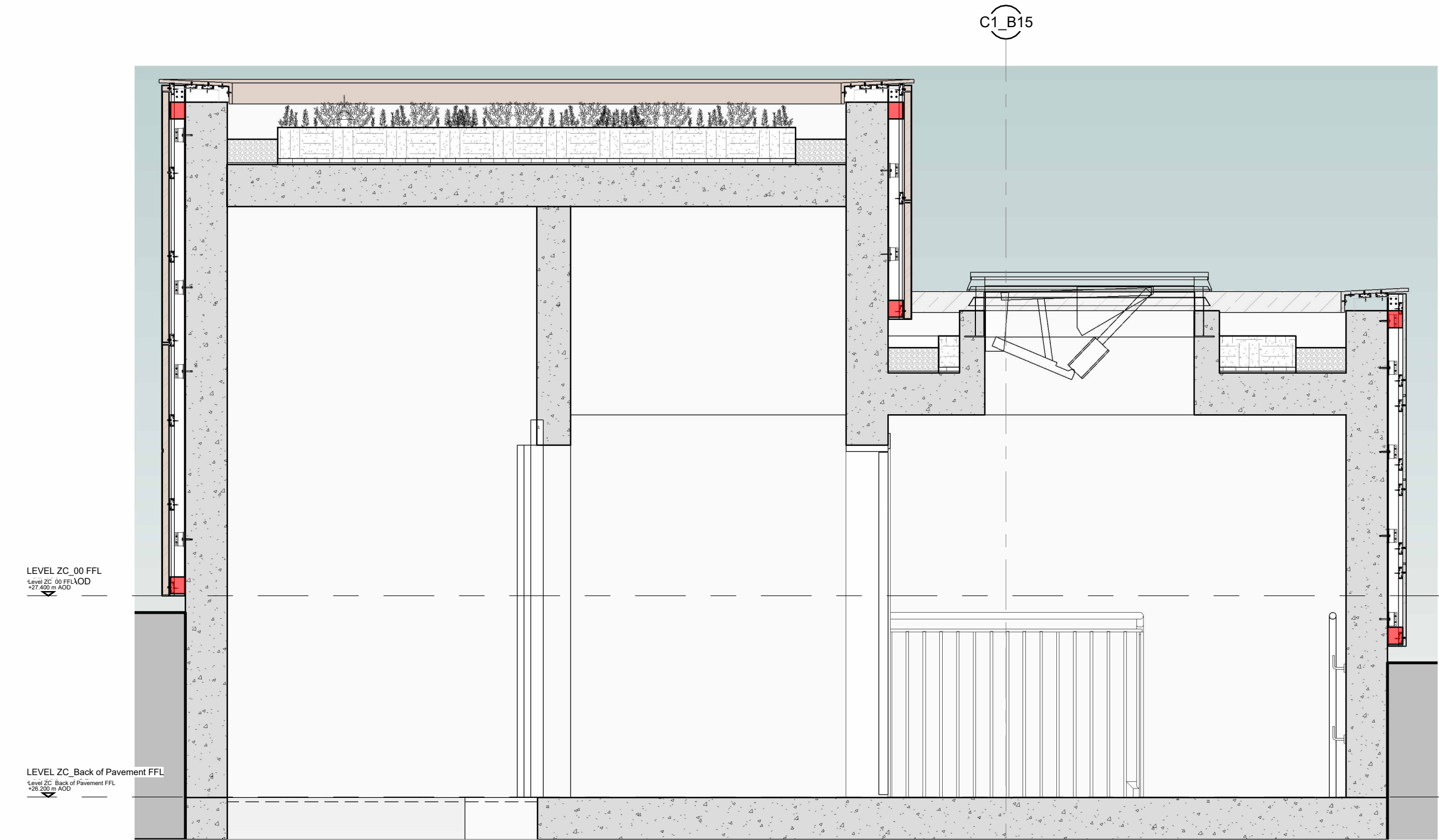
1 G251_C1_Core Pop Up_SE_AA 1 1 : 25
