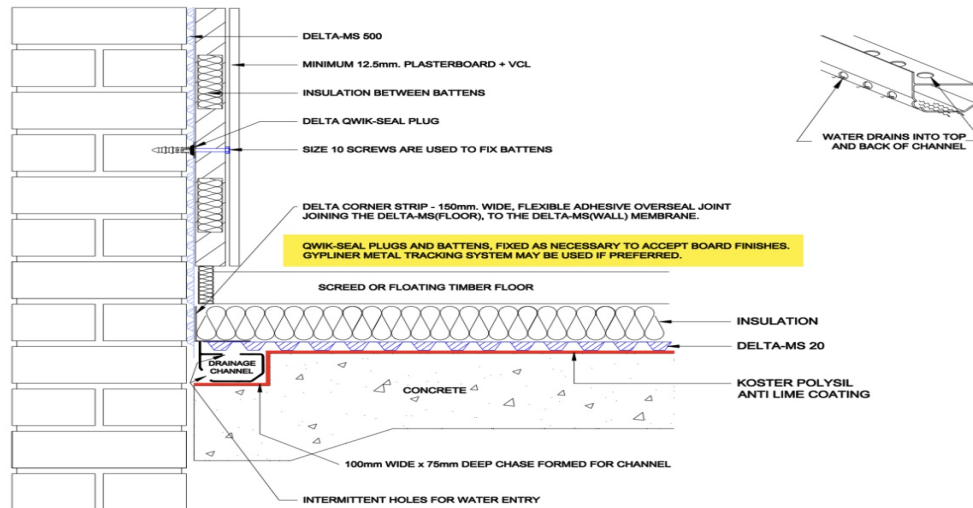
TYPE C, DRAINED PROTECTION, WALL AND FLOOR APPLICATION
