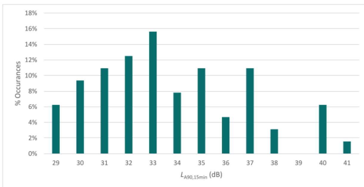
Figure 3: Statistical analysis of background sound pressure levels, nighttime
