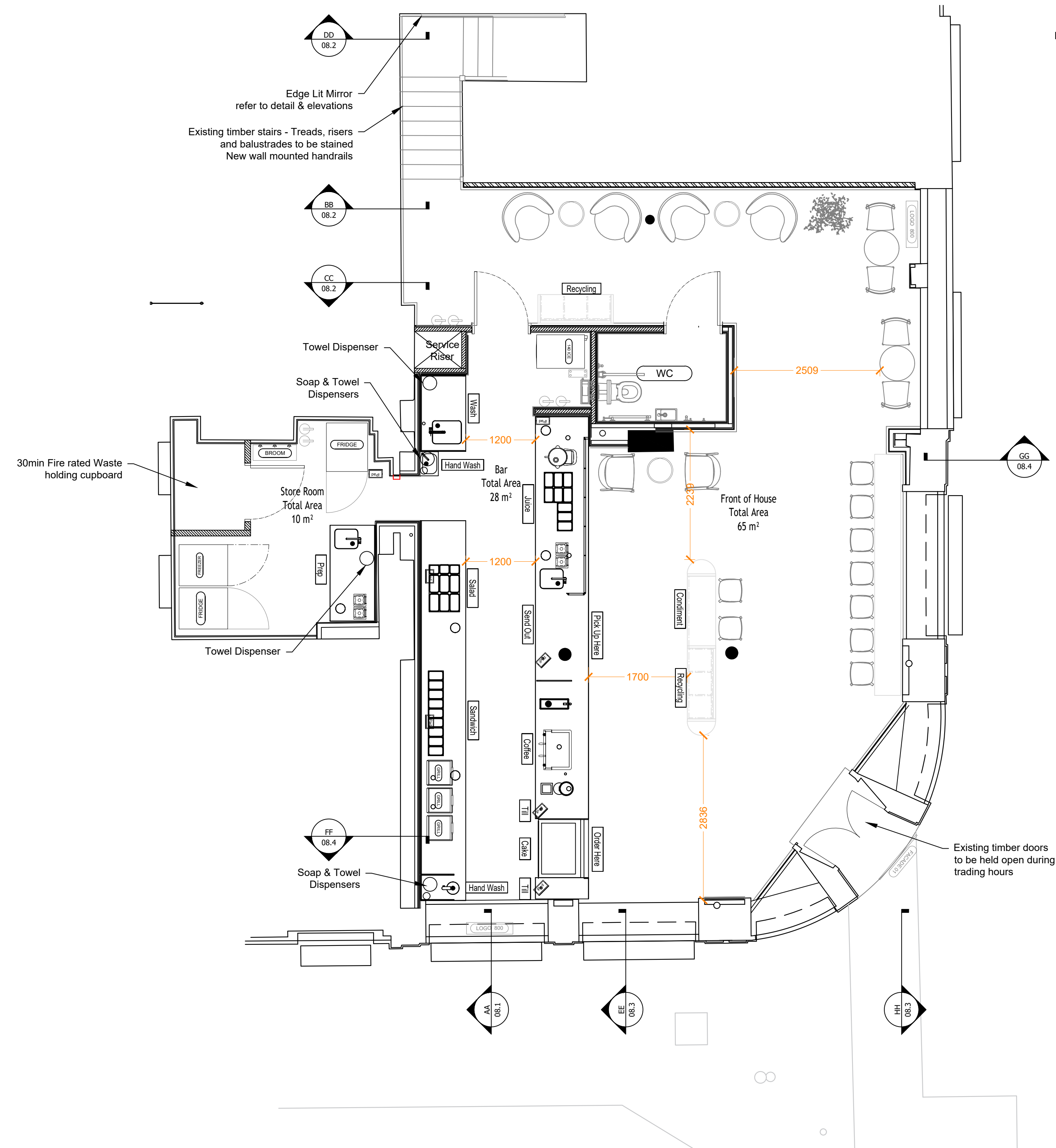
01 Ground Floor | General Arrangement Plan
