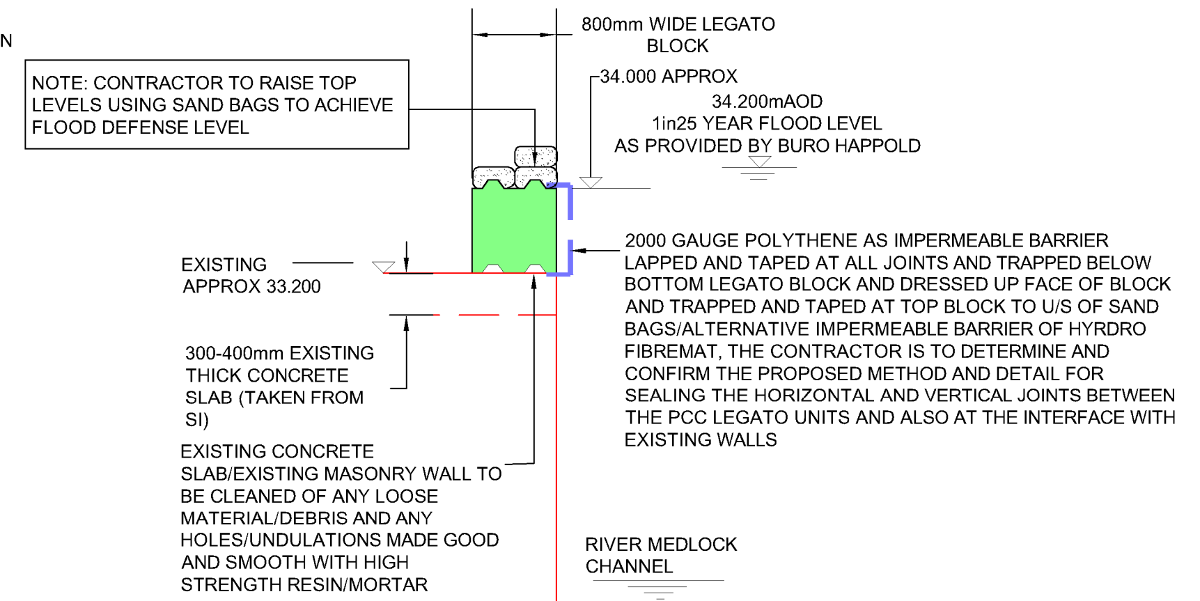
SECTION THROUGH WALL AT APPROX CHAINAGE 20 ON ELEVATION 1 SCALE 1:50
