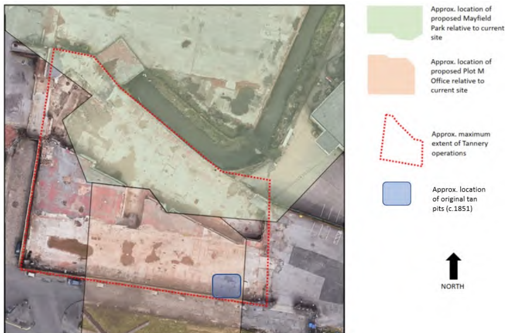
Fig 3.1: Approx. former Tannery Extent (red dashed line) General Remedial Comments
