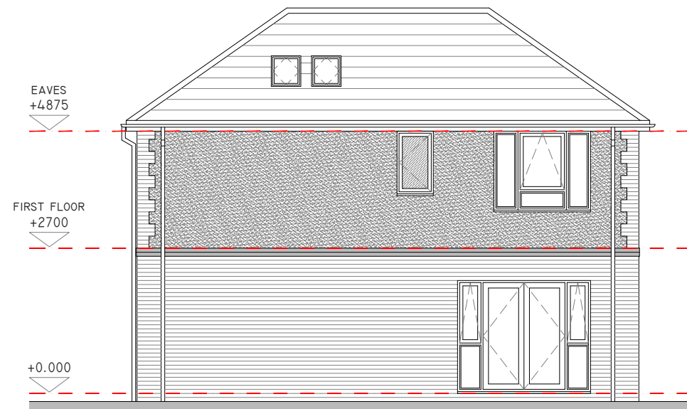
EAST ELEVATION
