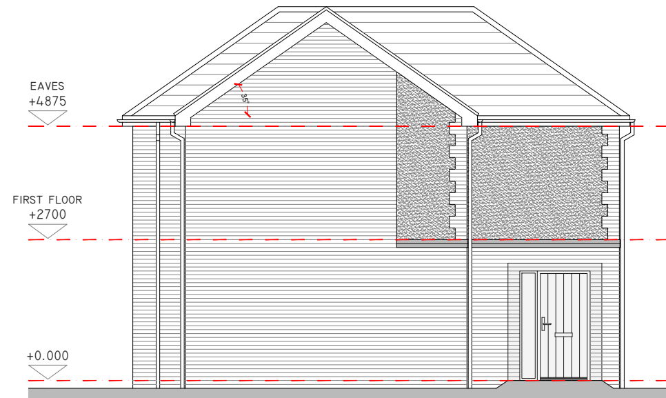
WEST ELEVATION
