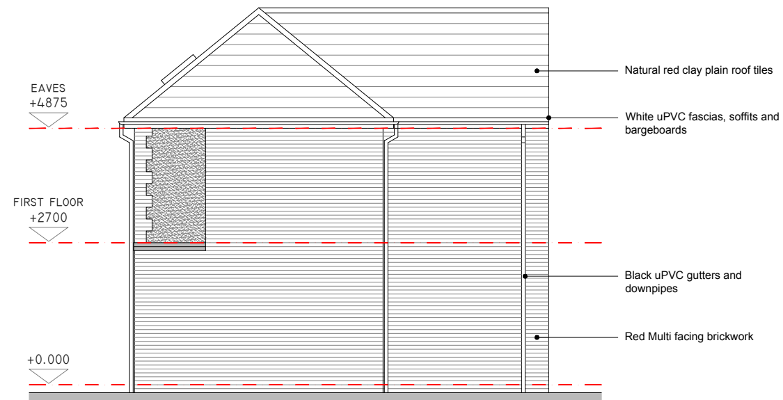
NORTH ELEVATION
