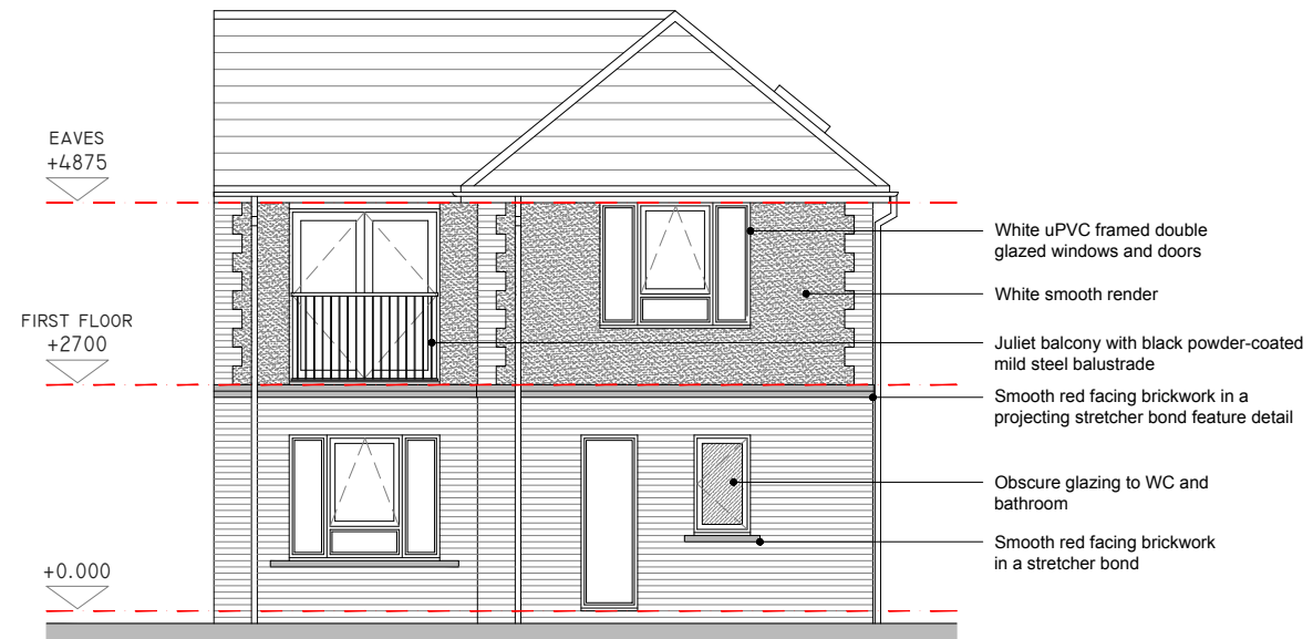
SOUTH ELEVATION
