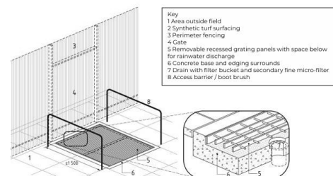
Example Detox grate outside a 3G pitch
