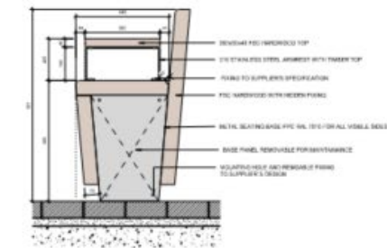
5 EXT-307 REMOVABLE BENCH SIDE ELEVATION 580mm 1:10
