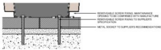
7 EXT-305 REMOVABLE BENCH FIXING DETAIL 1:4
