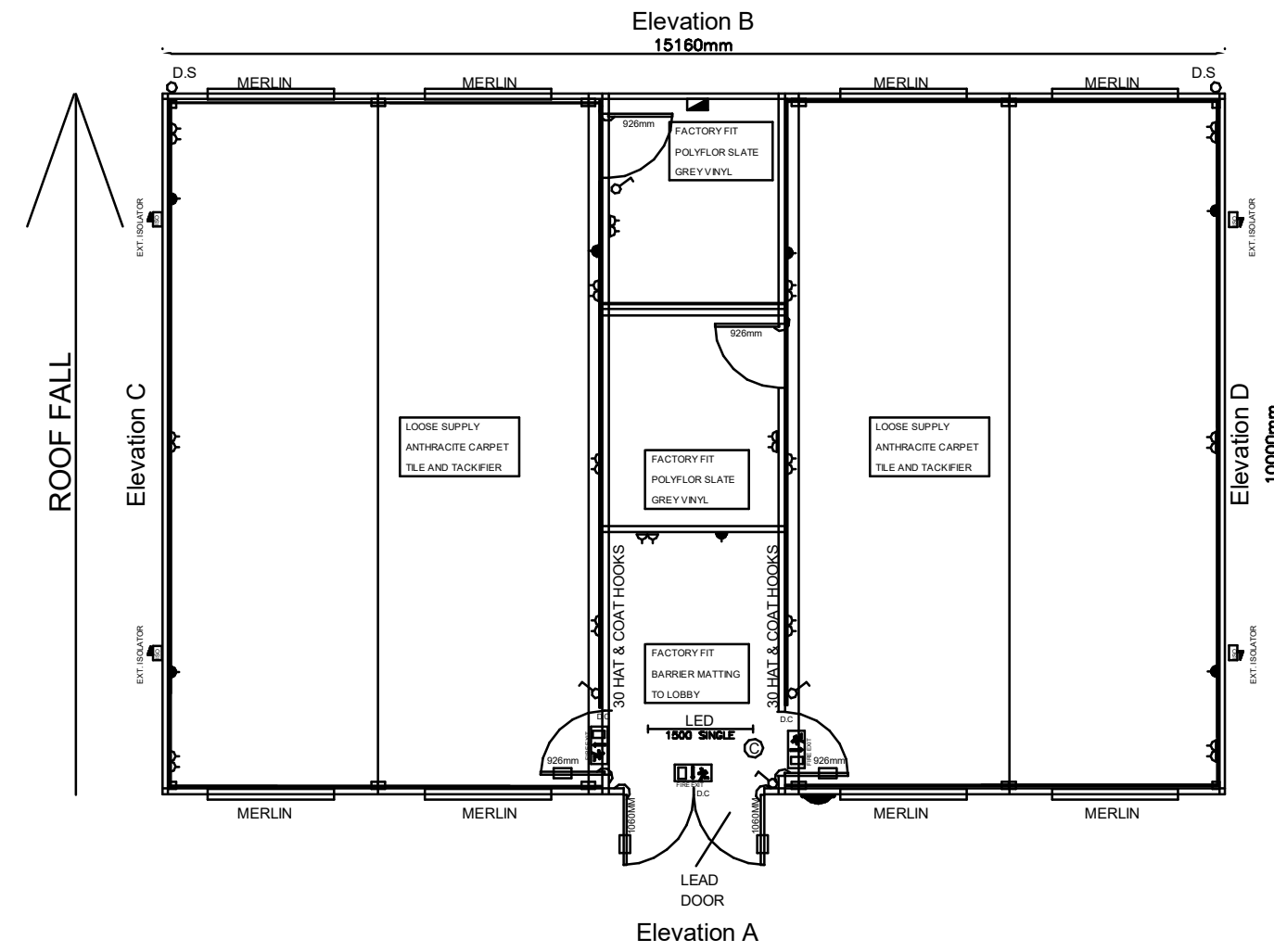
2 Unit A & B Plan 1:100
