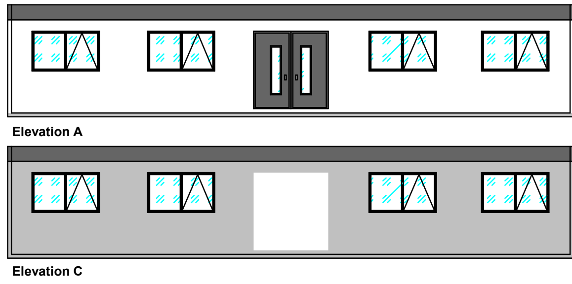
1 Unit A & B Elevations 1:100
