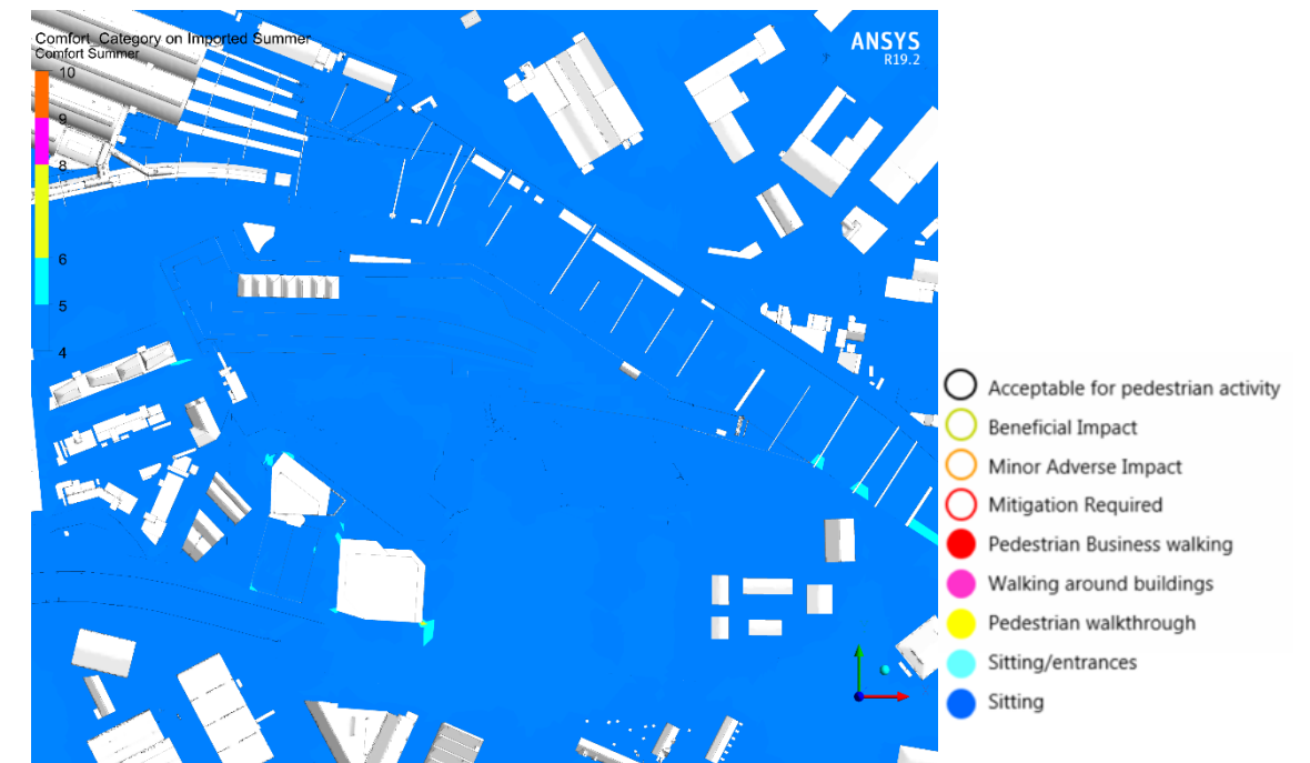
Figure 1-9 Cumulative scenario 1: Phase 1 Application 1 + Application 2 in future surroundings - summer composite comfort map (12 wind directions)
