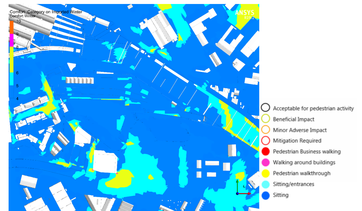
Figure 1-10 Cumulative scenario 1: Phase 1 Application 1 + Application 2 in future surroundings - winter composite comfort map (12 wind directions)
