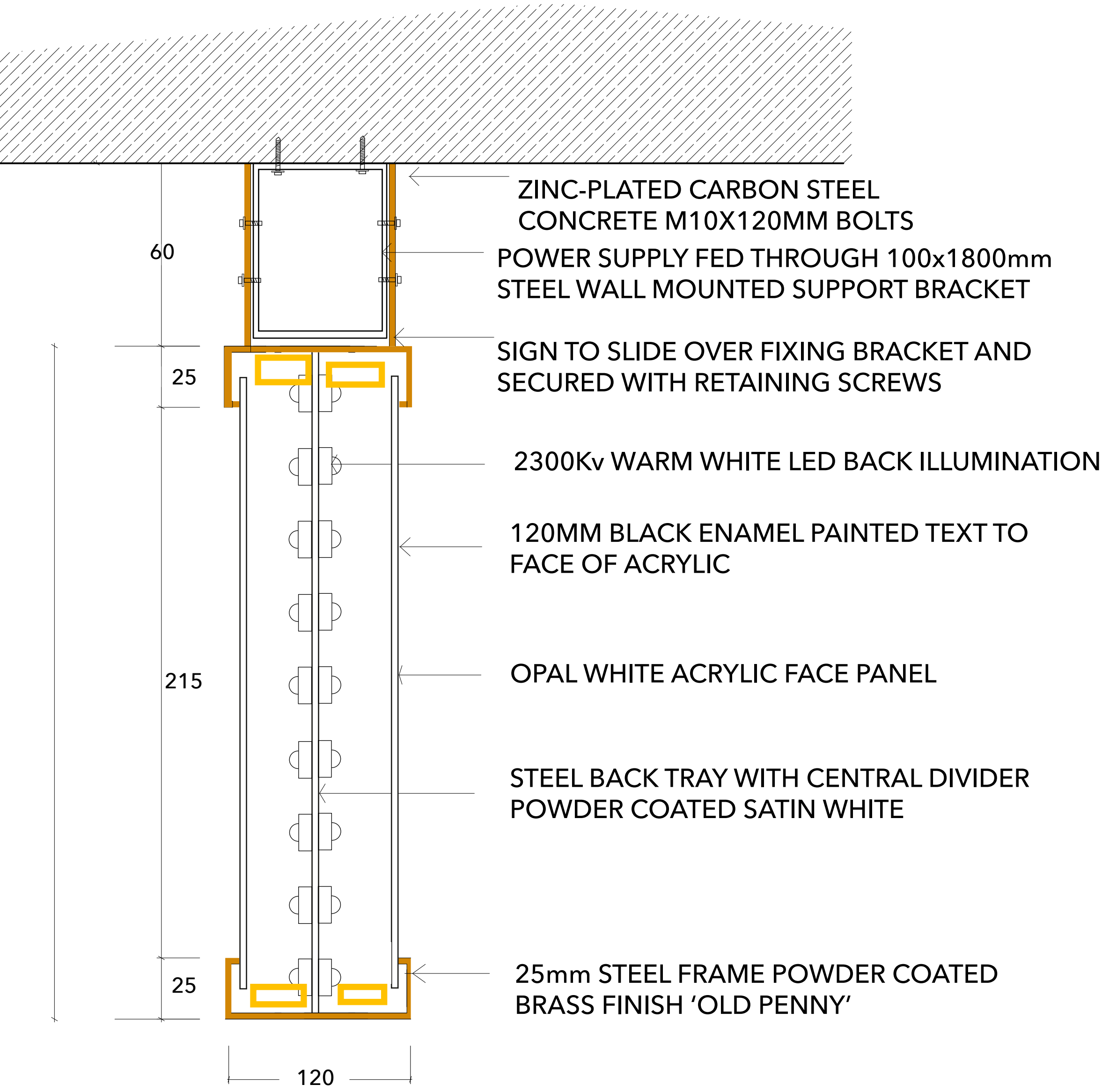
SECTION DETAIL
