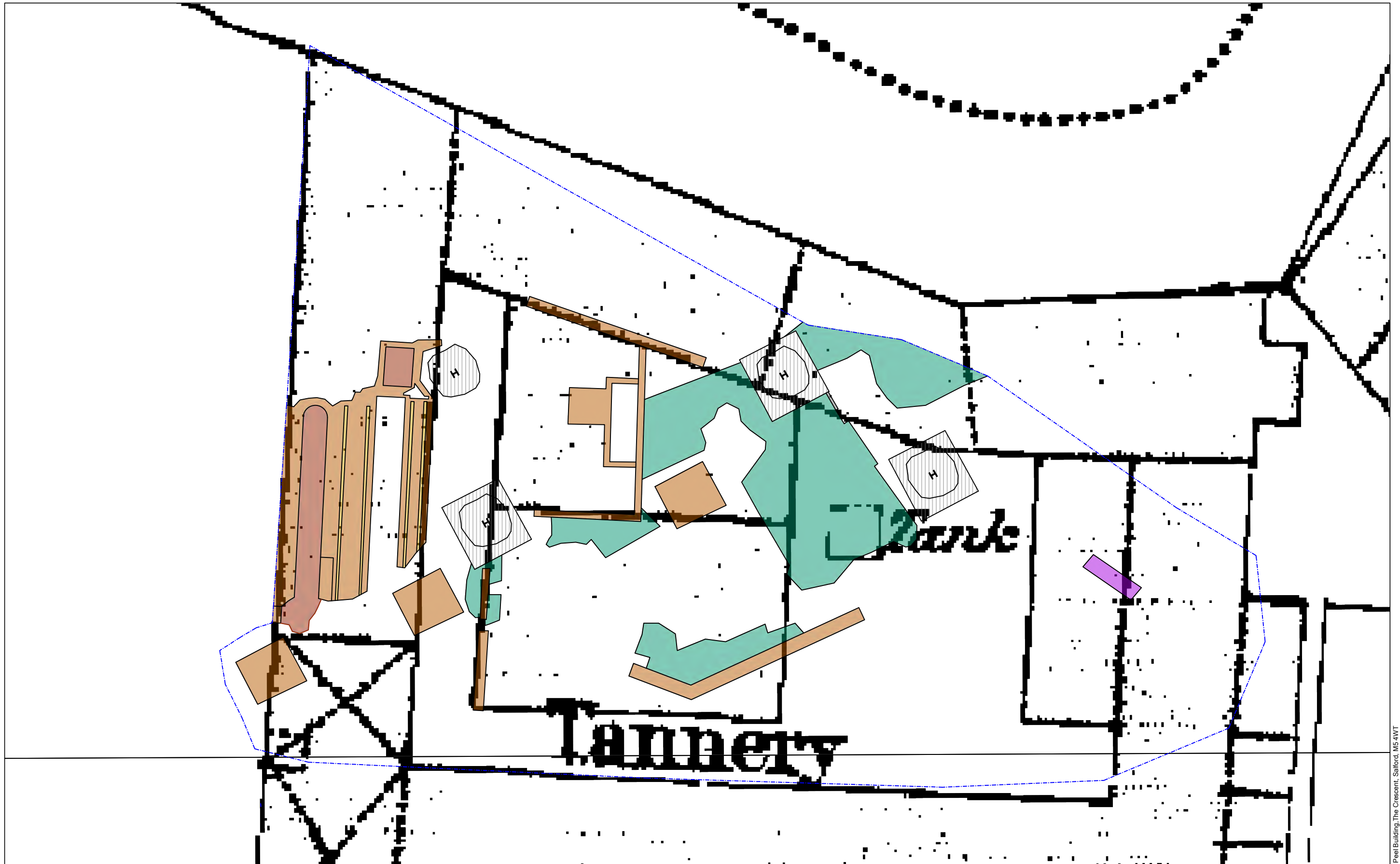
Figure 5: Area 1 Excavated remains superimposed onto the 1:1056 Town Plan of 1851 Contains Ordnance Survey data © Crown copyright and database right 2021
