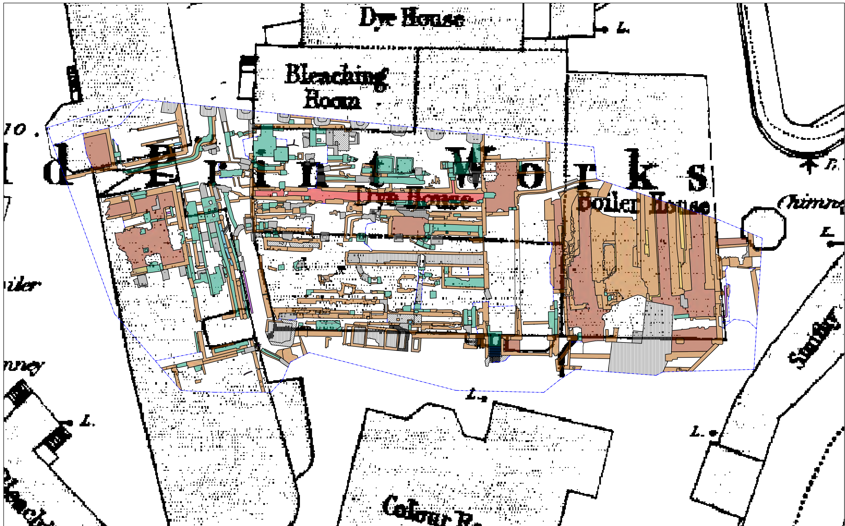
Figure 16: Area 3 Excavated remains Superimposed onto the 1:1056 Town Plan of 1851
