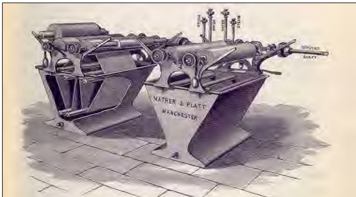
Plate 198: Dye jigger
