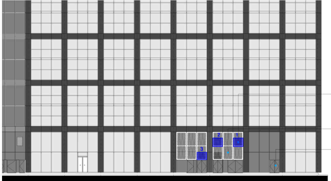
Figure 3 Excerpt of drawing SF-24013-07 showing the proposed grille terminations to the east elevation (in blue)
