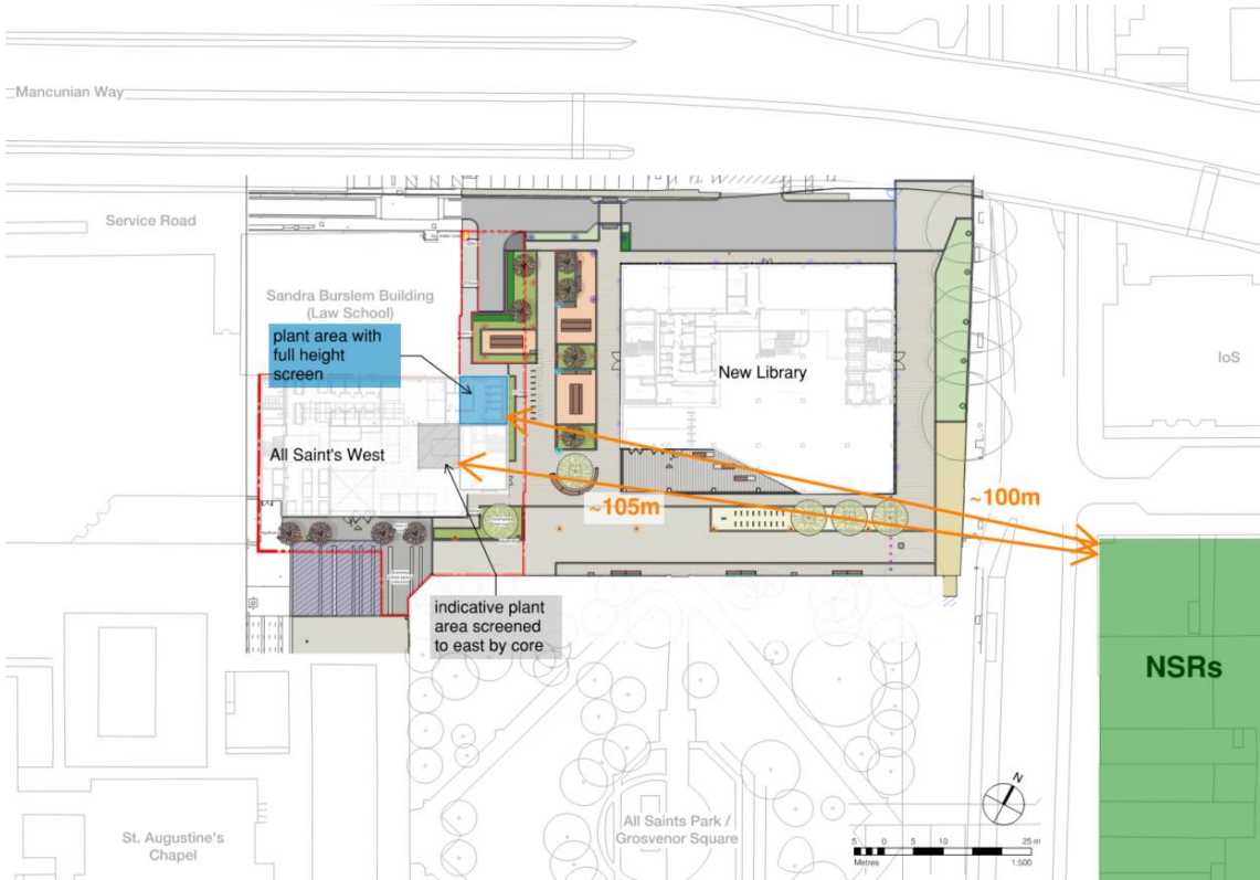
Figure 5—2 Mark up indicating plant locations and NSRs (source: 103040-PLA-XX-XX-DR-L-0001 overlayed onto 1350B-HBA-XX-RF-DR-A-200004)
