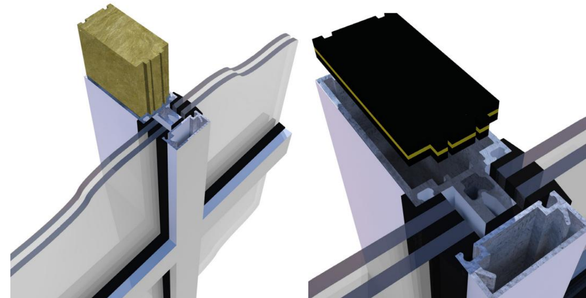
Figure 4—2 Siderise MF Insert (left) and Siderise AVC M11 closure (right)
