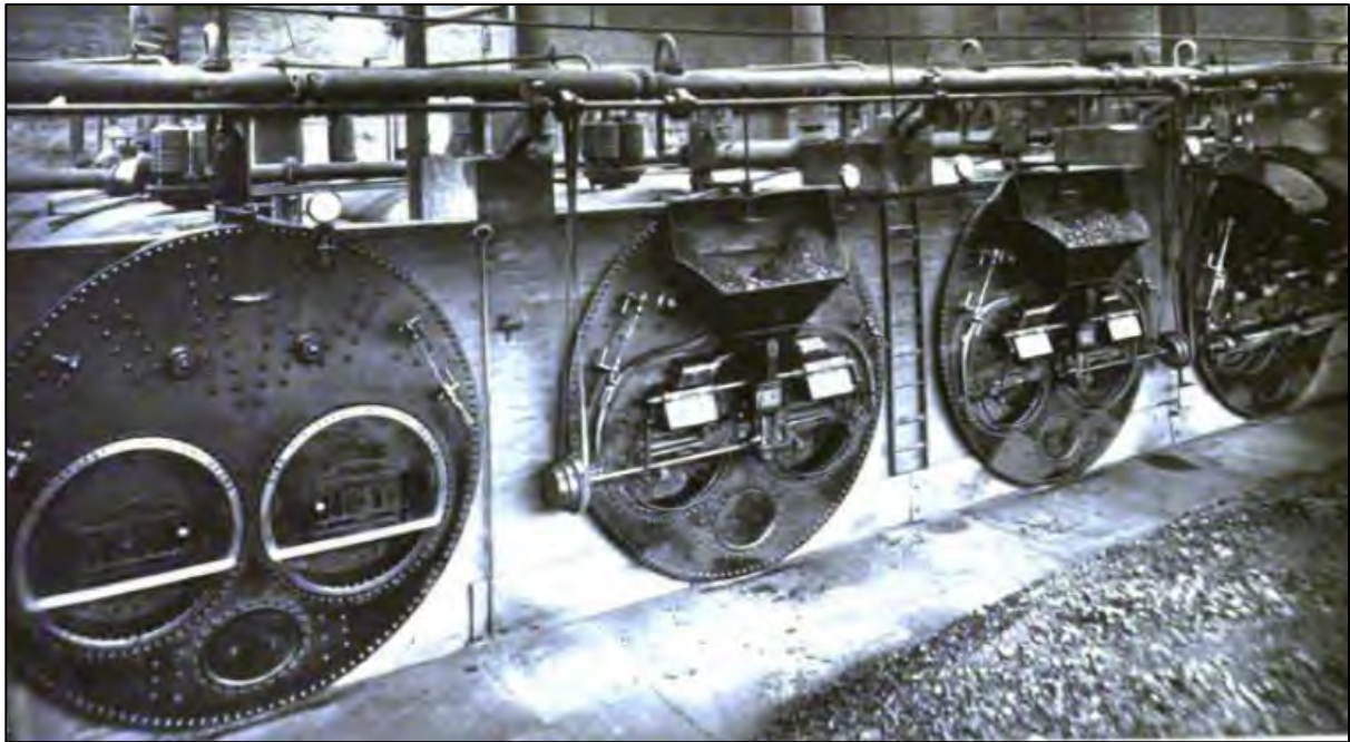
Plate 204: An example of a bank of Lancashire boilers, some fitted with automatic feeders (hoppers
