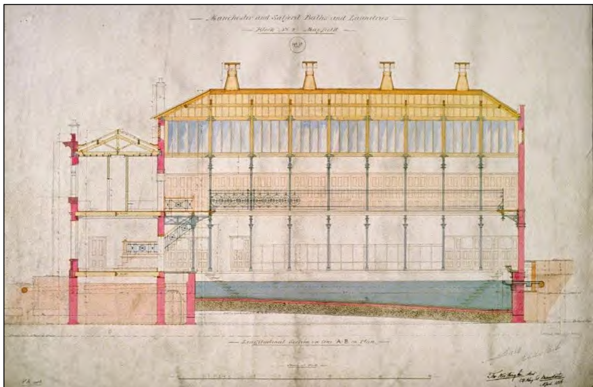
Plate 181: Worthington's design plan of Mayfield Baths, drawn on canvas by Thomas Worthington in April 1856
