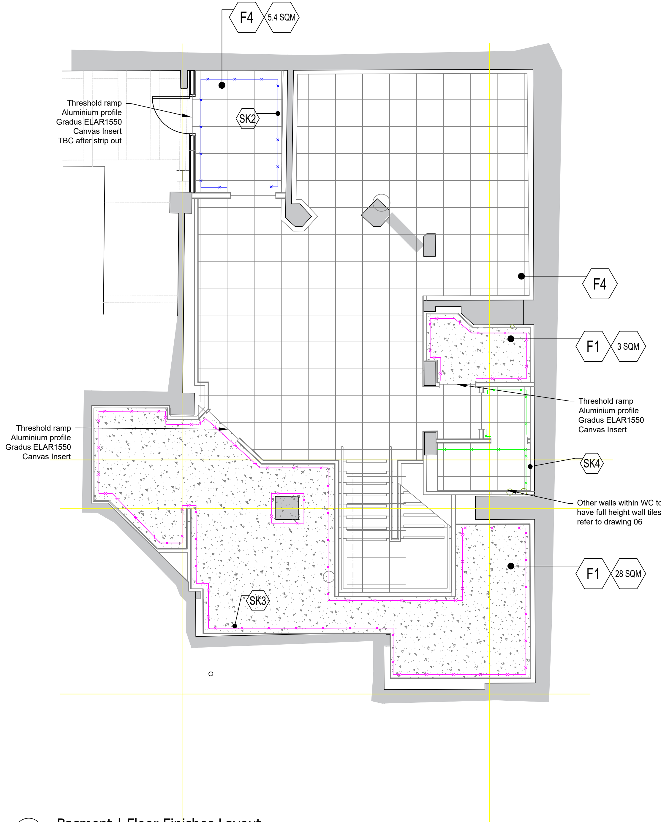
07 Basment | Floor Finishes Layout
