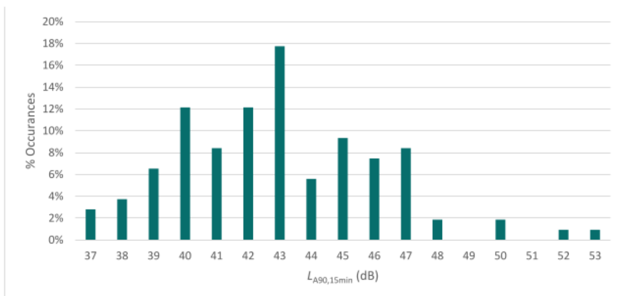
Figure 2: Statistical analysis of background sound pressure levels, daytime
